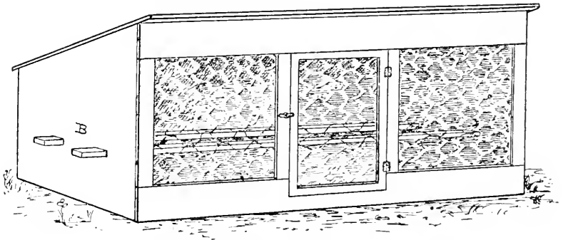
Fig 10. Coop B.—Length, 6 ft. : width, 2 ft. 6 in. : height \frac{1}{2} in front, 2 ft. 4 in. : height at back, 18 in.
