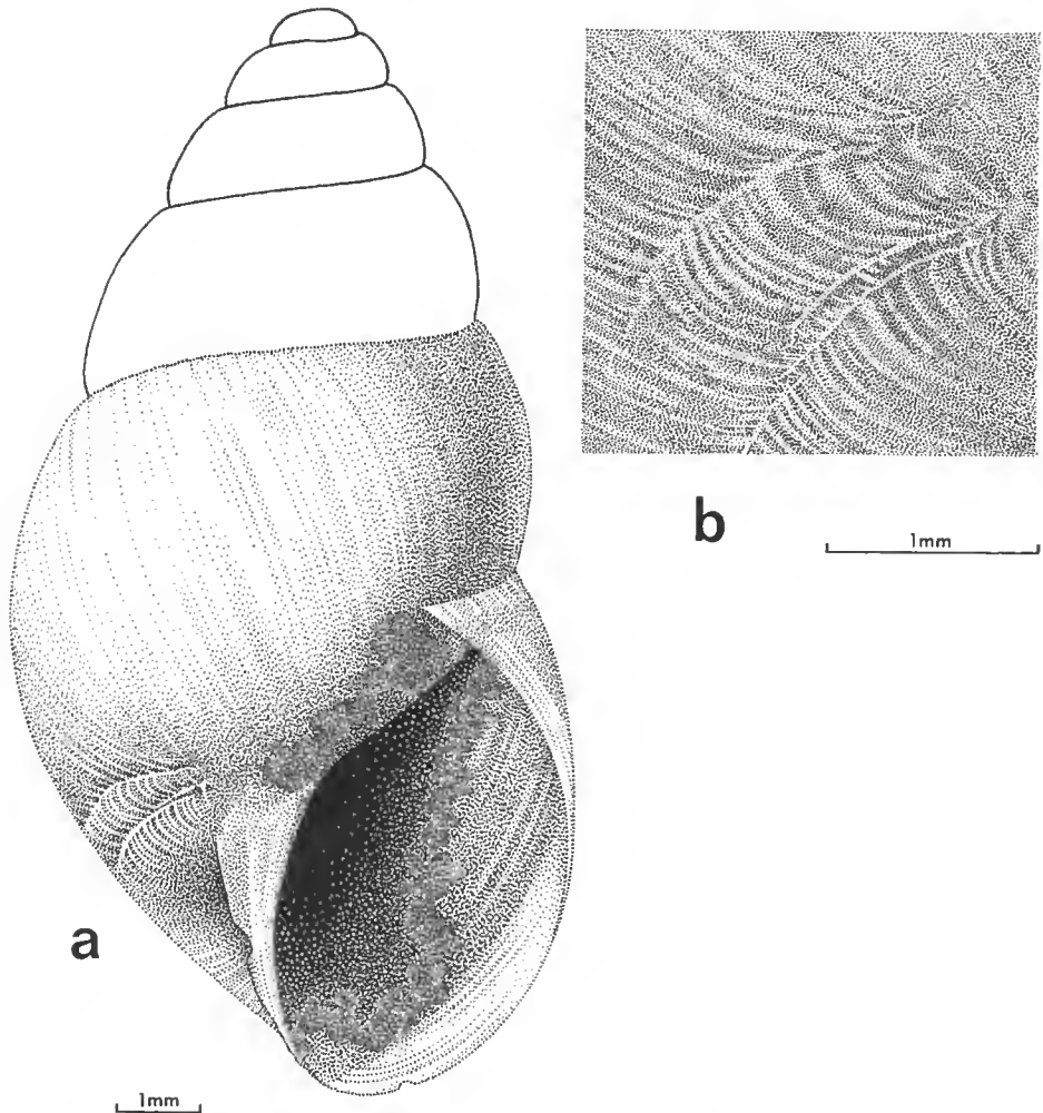
TEXT-FIG. 1. — Peronaeus limonoicus (d'Orbigny), lectotype. H. Heijn del. a, outline of shell; b, detail of sculpture on last whorl.
