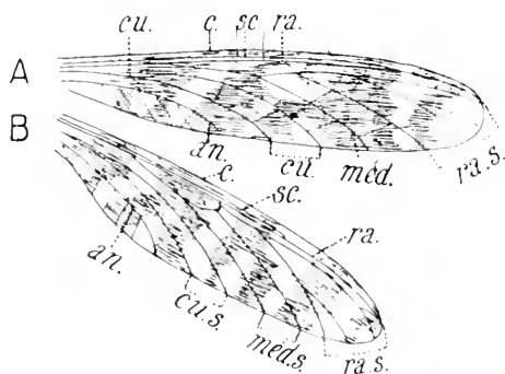
Fig. 4. — Restauration de Sphecopectera Brongniarti nov. sp.
