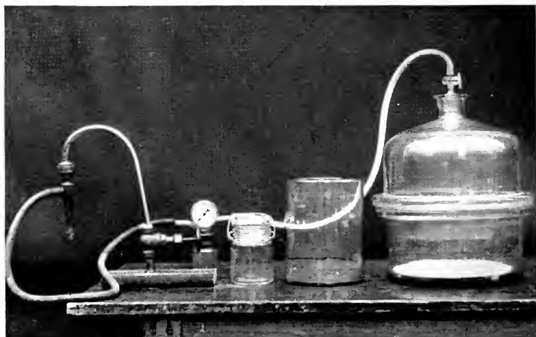
Plate III. Apparatus for the Determination of Vacuums by the Vacuum Desiccator Method.
