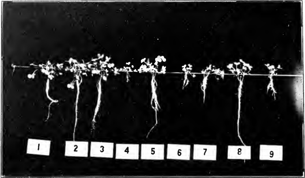
No. 1, Nutrient sol.; No. 2, Nutrient sol.+CaCO 3 ; No. 3, Nutrient sol.+CaSO 4 ; No. 4, Nutrient sol.+2 e.c. Al sol.; No. 5, same as No. 4+CaCO 3 ; No. 6, same as No. 4+CaSO 4 ; No. 7, Nutrient sol.+1 e.c. Al sol.; No. 8, same as No. 7+CaCO 3 ; No. 9, same as No. 7+CaSO 4 .
