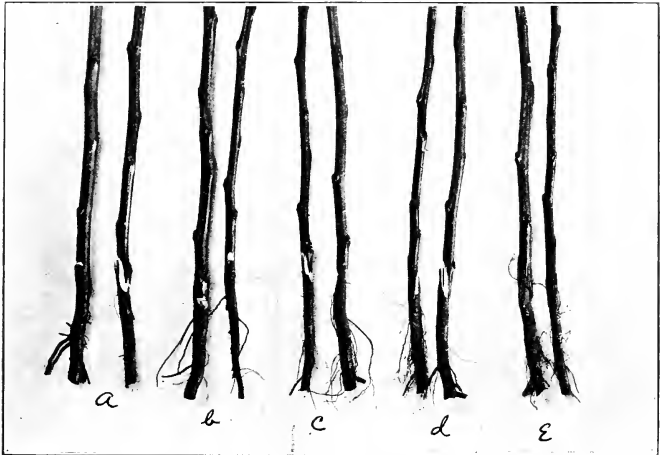
FIG. 2. — Matching cambium in root grafts: (a) one side only; (b) both sides only; (c) top only; (d) bottom only; (e) perfectly matched.
