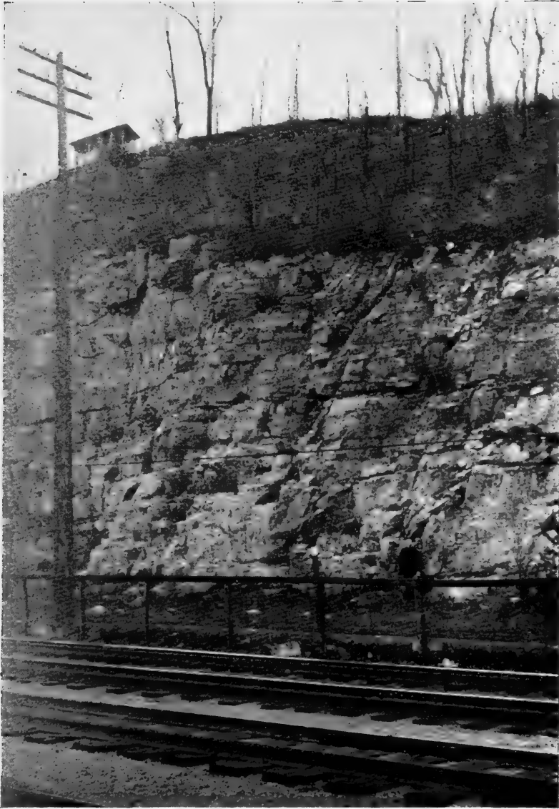
RAILROAD CUT IN CALCIFEROUS SANDSTONE AT HOFFMANS
