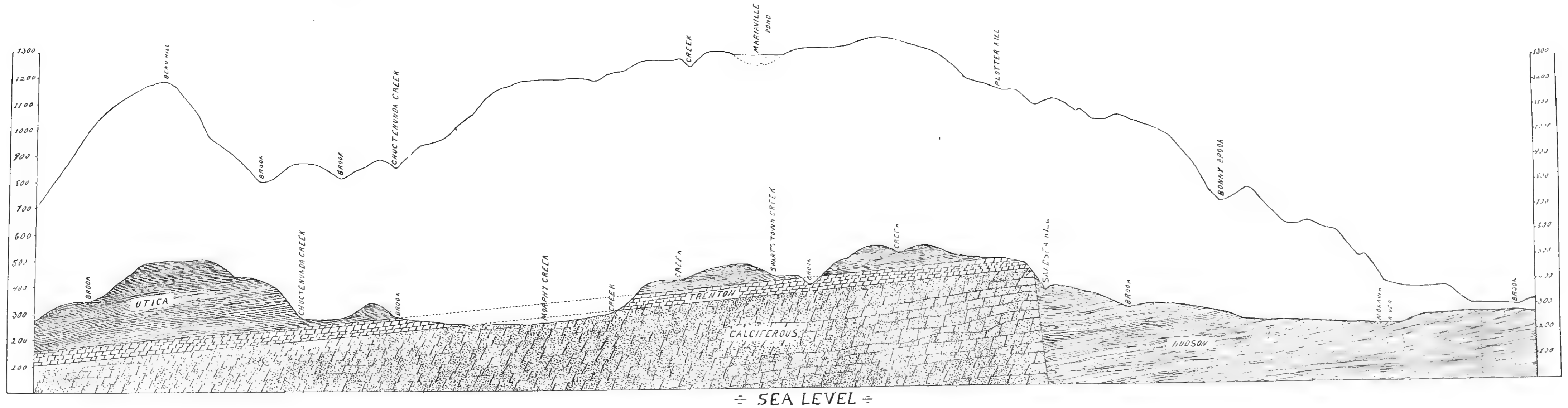
A SECTION ACROSS THE AMSTERDAM SHEET JUST SOUTH OF THE MOHAWK RIVER AND A PARALLEL SECTION FIVE AND ONE HALF MILES TO THE SOUTH.
