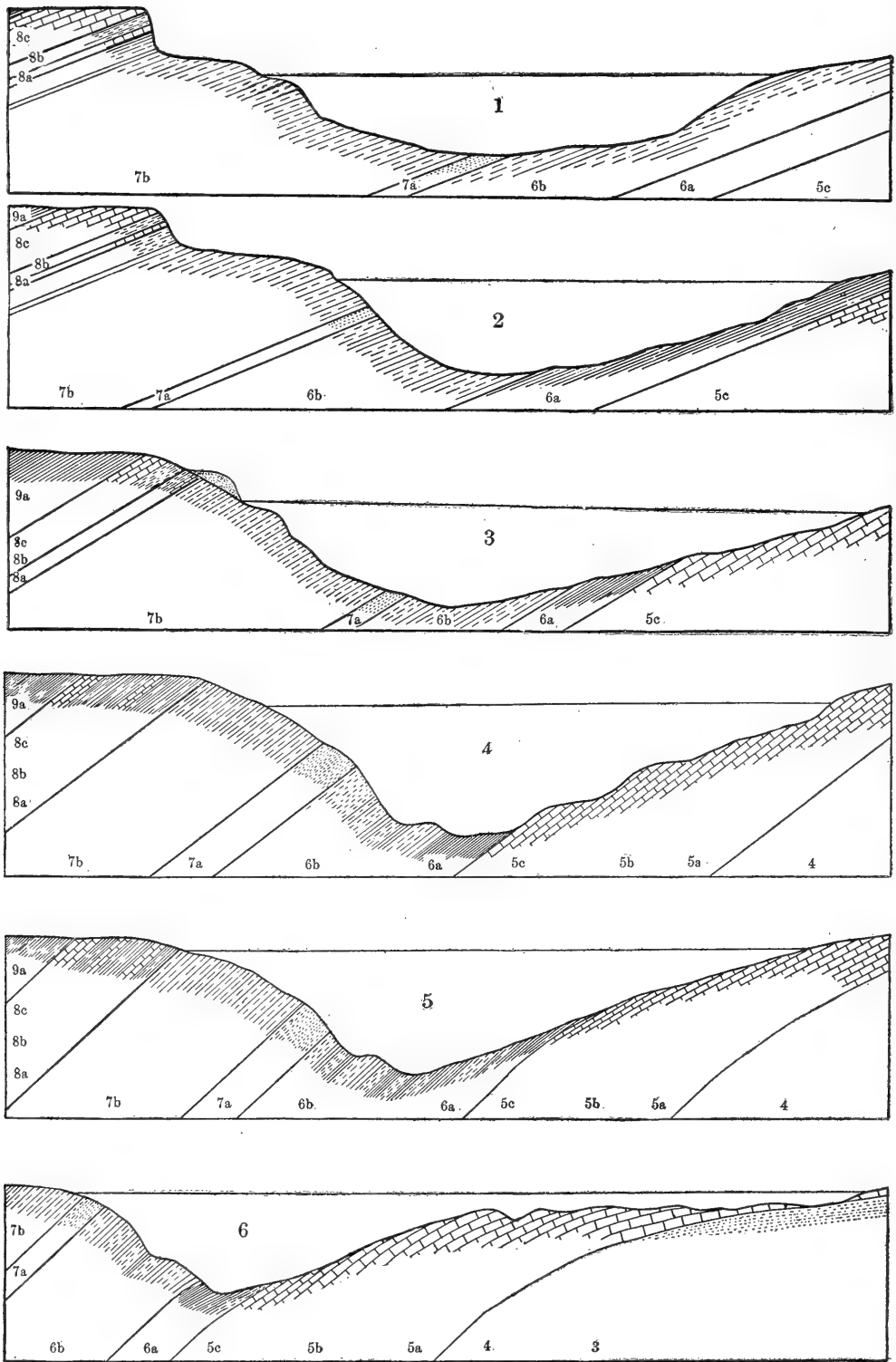
Fig. 7 Six cross-sections of Lake Ontario showing topography and geology. Vertical scale 1 inch = 1280 feet; horizontal scale 1 inch = 15\frac{3}{4} miles. Numbering of beds as in table; location of sections indicated in fig. 5. Section 1) E. of Niagara to E. of Pickering light. 2) Lockport to Darlington light. 3) West of Genesee to Presque Isle light. 4) Pultneyville to Point Peter. 5) West of Fair Haven light to False Buck light. 6) Oswego to Kingston.
