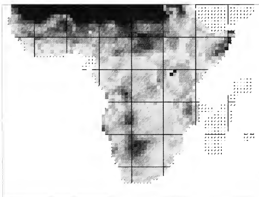
Fig 1b. Map of bird species-endemism in Afrotropical Africa (based on computerised maps compiled from a variety of sources). Darkest areas = areas of low endemism scores for birds (blue in original colour map, grading through green, yellow and finally red for the areas of increasing endemism scores).
