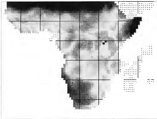
Fig 1a. Map of bird species-richness in Afrotropical Africa (based on computerised bird species distribution maps compiled from a variety of sources). Darkest areas = areas of low richness for birds (blue in original colour map, grading through green, yellow and finally red for the areas of increasing species richness).
