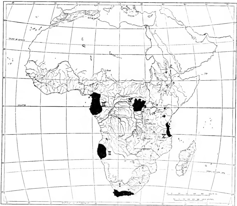
Map 16. Genera of Lacertidae in Africa with restricted distribution: I, Tropidosaurosa ; II, Aporosaurosa ; III, Paromera ; IV, Bedriagaia ; V, Gastropholis .
