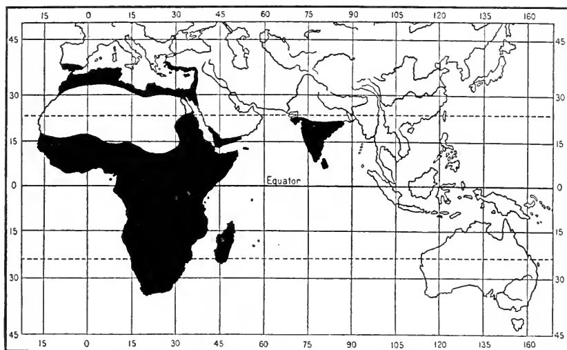
Map 18. Distribution of the Chamaeleontidae.
