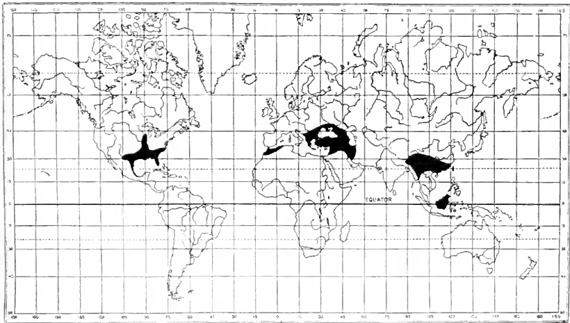
Map 12. Distribution of the genus Ophisaurus (Anguillidae).
