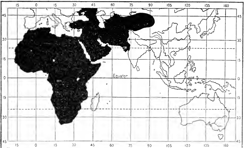
Map 9. Distribution of the genus Agama (Agamidae). Maps 7, 8, and 9 illustrate hypothetical stages in the invasion of Africa by the Agamidae.
