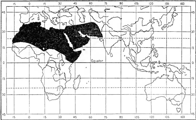
Map 4. Distribution of the genus Stenodactylus (Gekkonidae).
