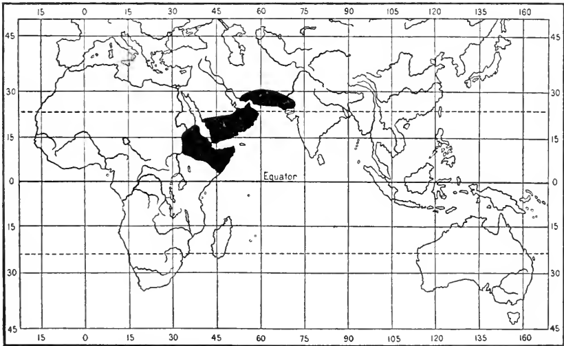
Map 5. Distribution of the genus Pristurus (Gekkonidae).
