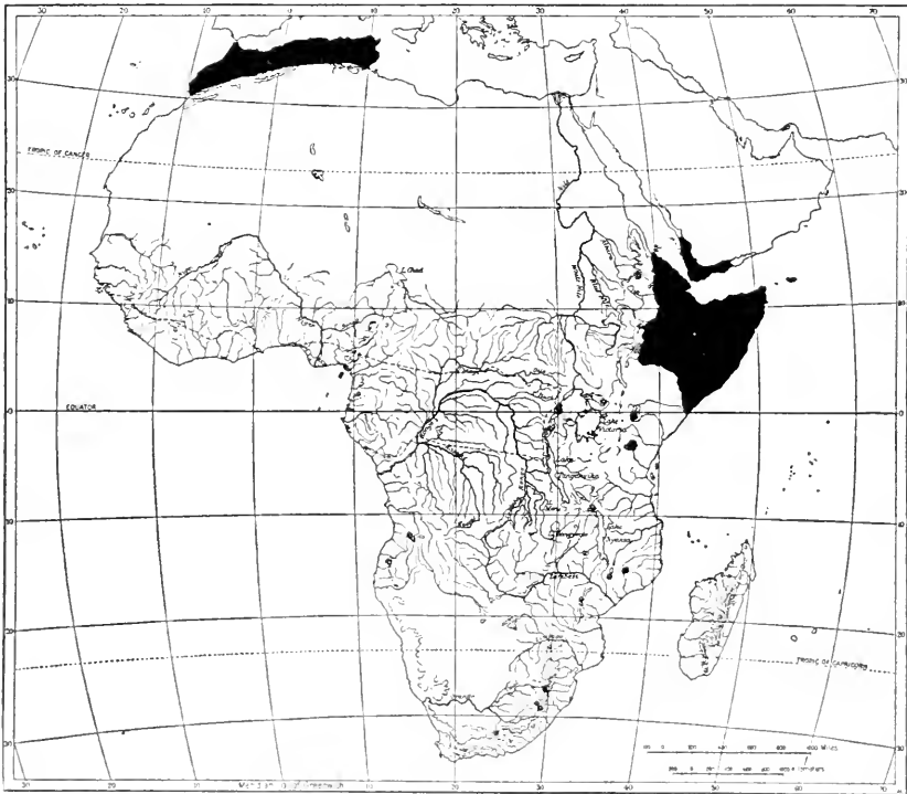
Map 14. Distribution of the section Emphyodontes (Amphispbenidae).
