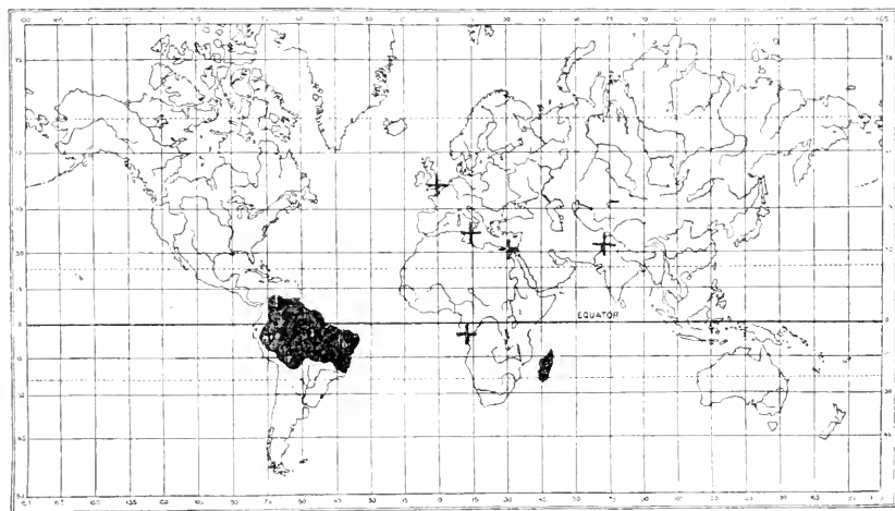
Map 3. The present and past distribution of the genus Podocnemis of the Pelomedusidae.
