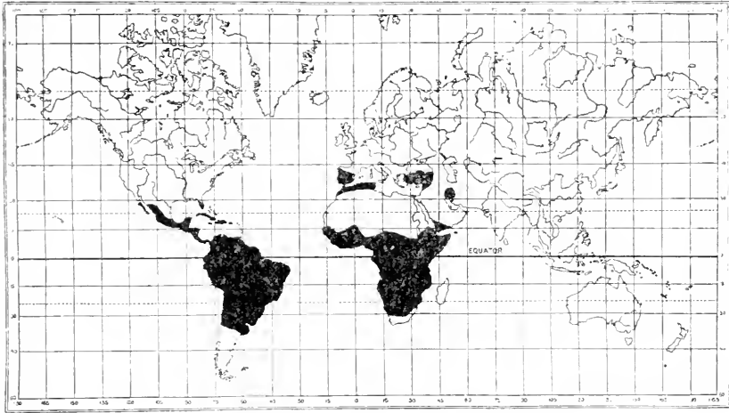
Map 13. Distribution of the Amphispbenidae.
