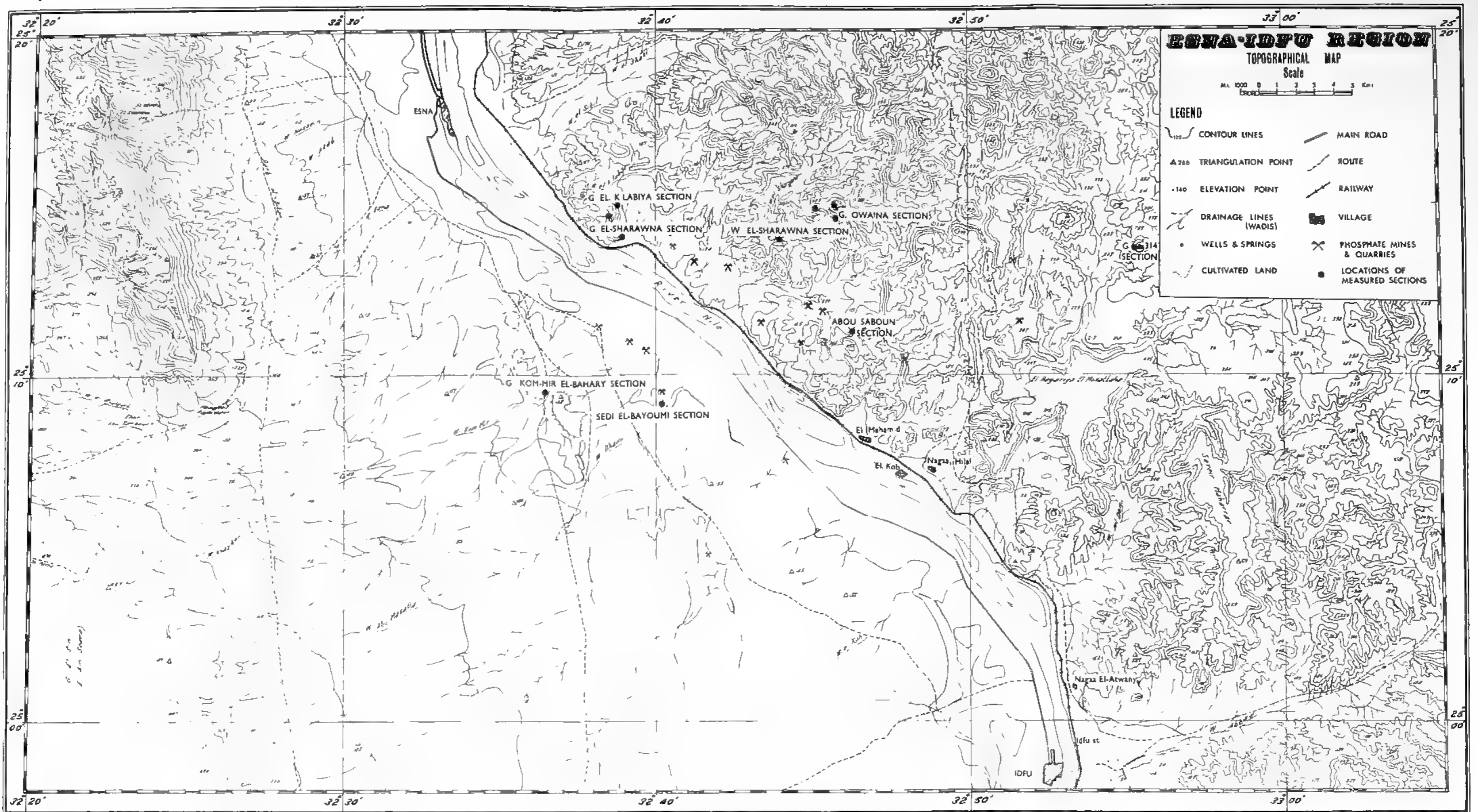
FIG. 2. Esna-Idfu Region Topographical Map
