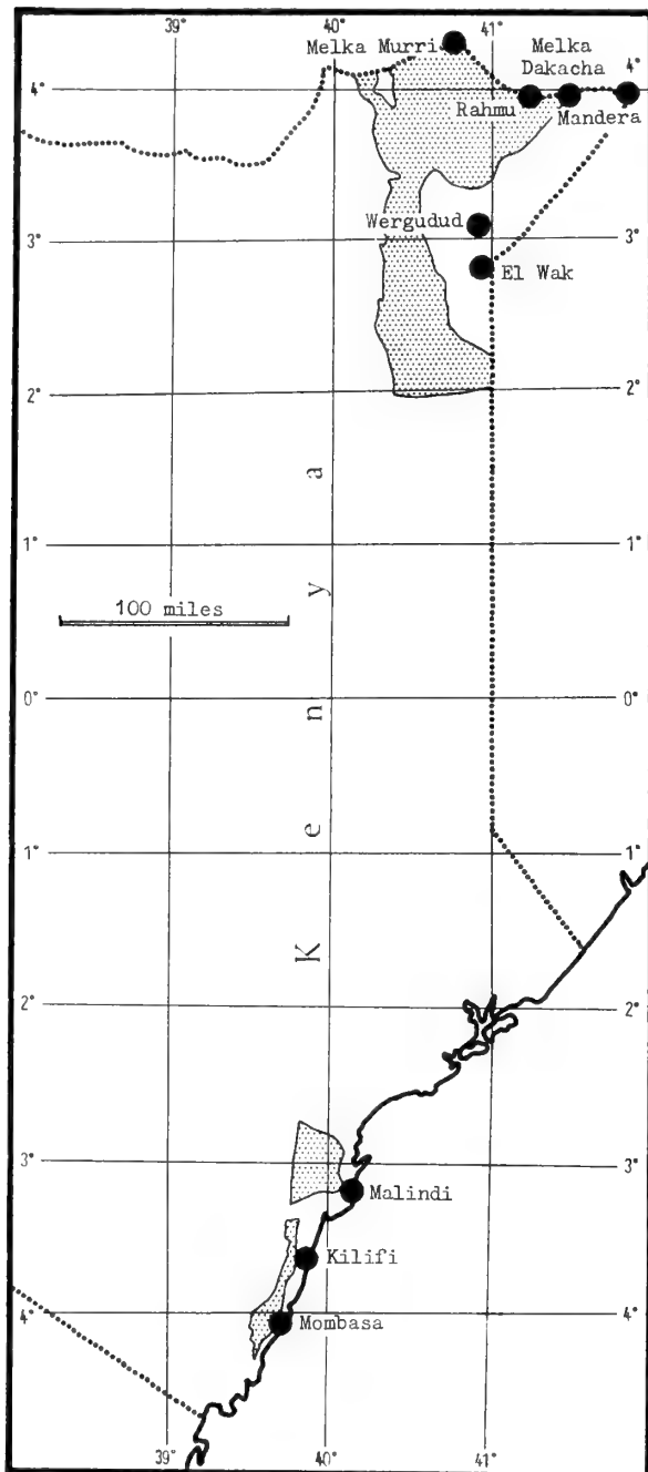
FIG. 2. Sketch-map of eastern Kenya, showing Jurassic outcrops.
