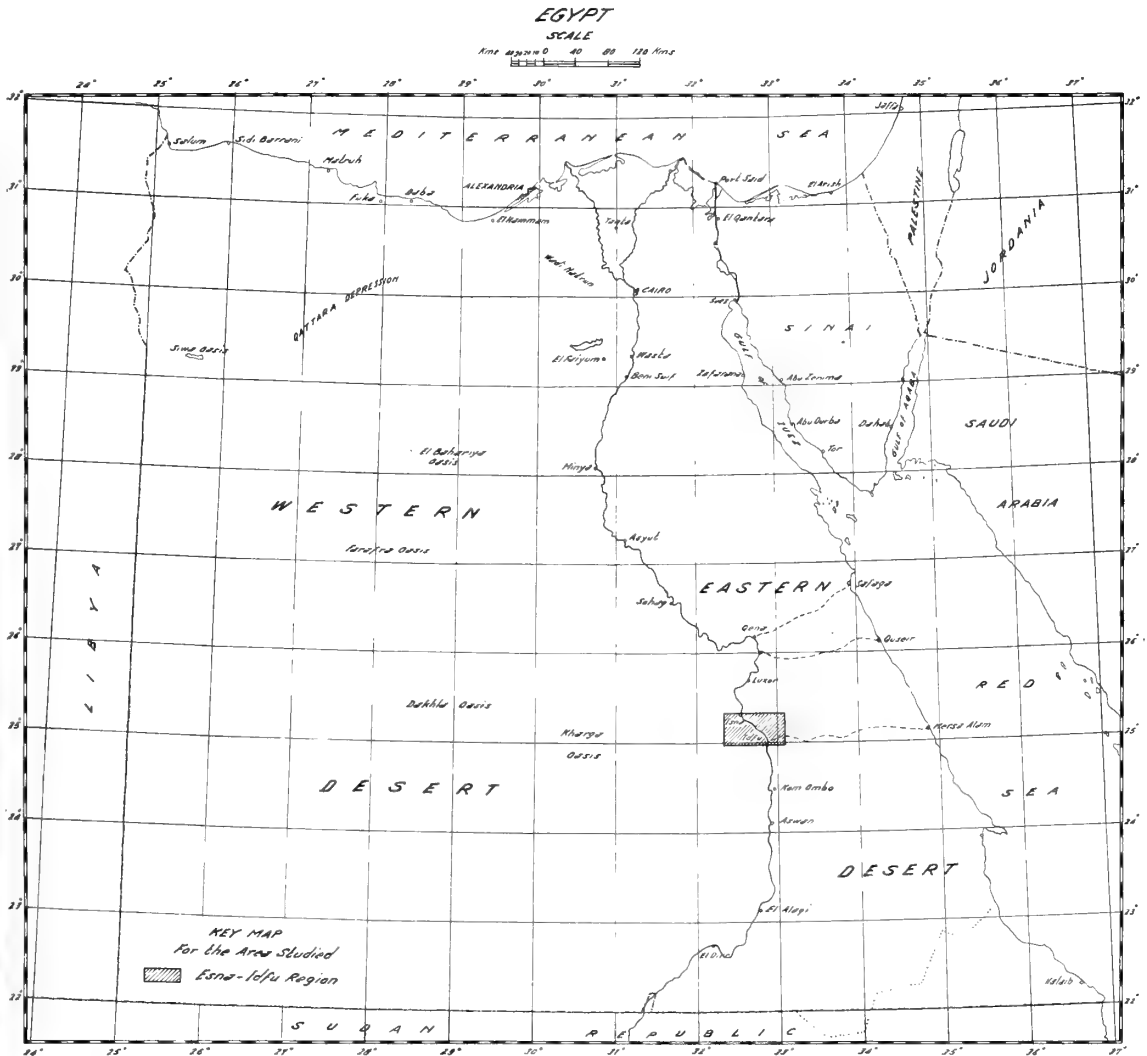
FIG. 1. Map of Egypt.
