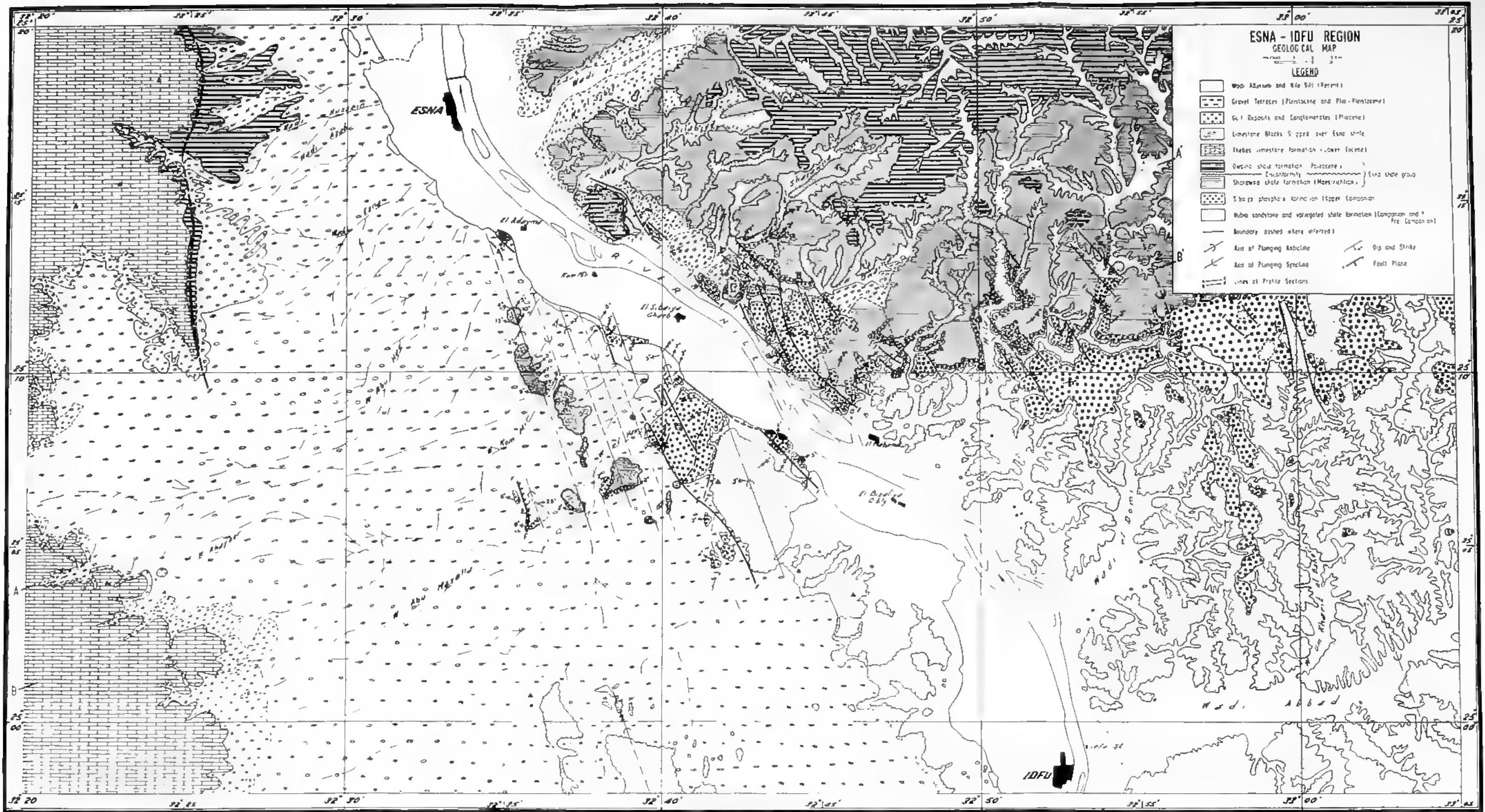
FIG 3. Esna Idfu Region Geological Map
