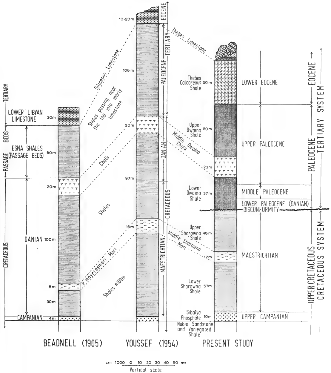
FIG. 4. Correlation of the stratigraphical succession in G. Owaina section as interpreted by Beadnell (1905), Youssef (1954) and by the present study.
