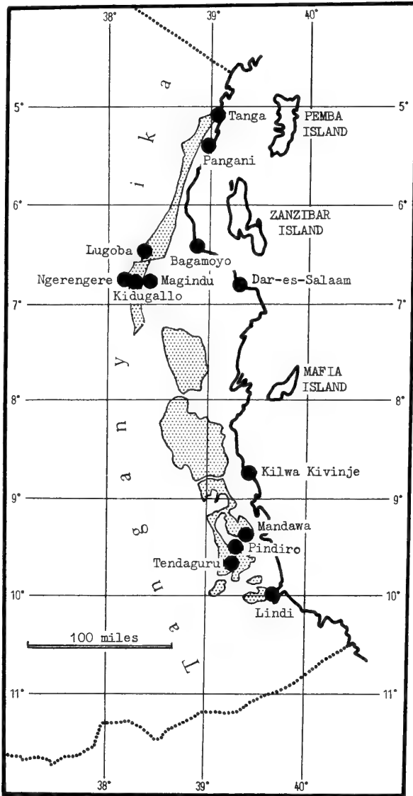
FIG. 1. Sketch-map of eastern Tanganyika, showing Jurassic outcrops.
