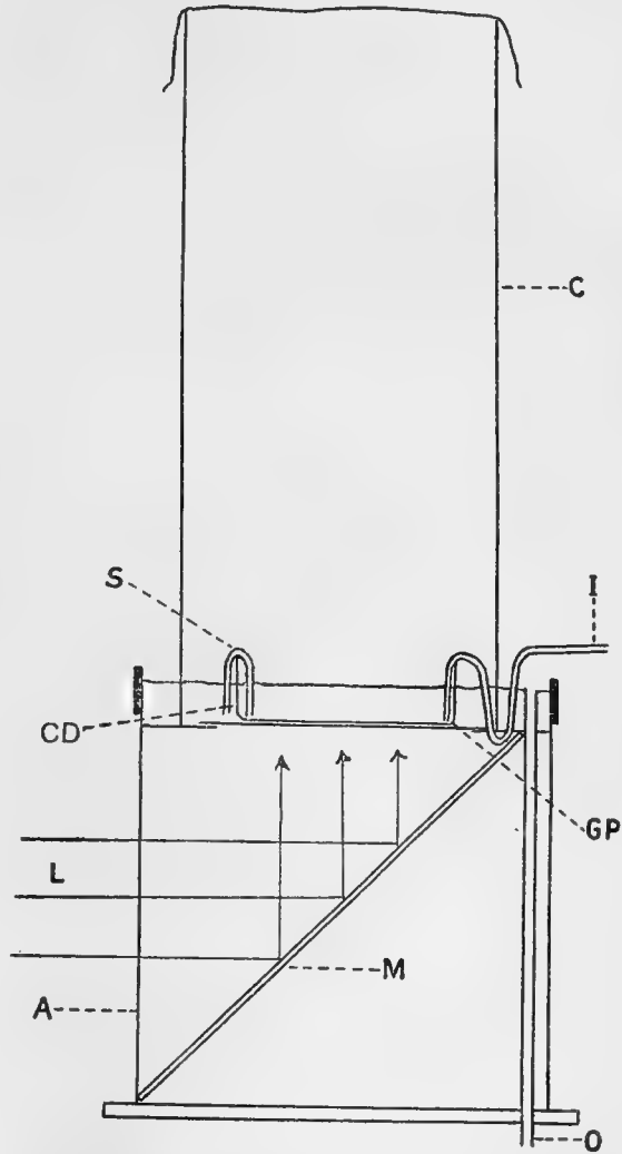
FIG. 2.—Vertical section of apparatus used in testing, in flounders, the effect of abnormally increasing the relative amount of light received by the eyes from below. A, glass aquarium; CD, crystalizing dish; S, siphon; I, inlet for water; O, outlet; GP, glass plate; C, opaque cylinder; M, mirror; L, light.
