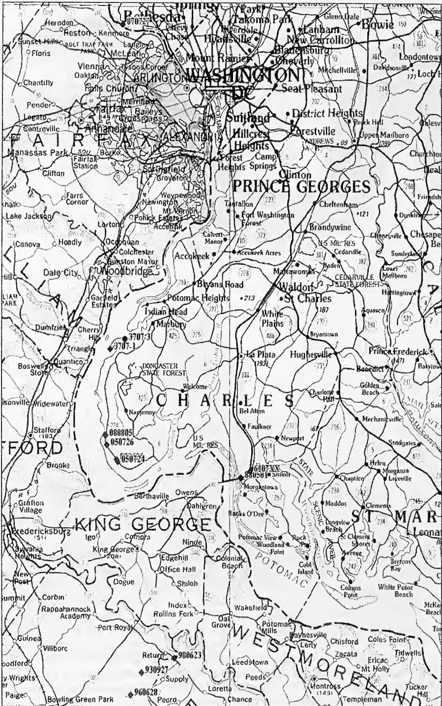
Fig 12. Regional Maryland and Virginia records for Farancia erytrogamma .
