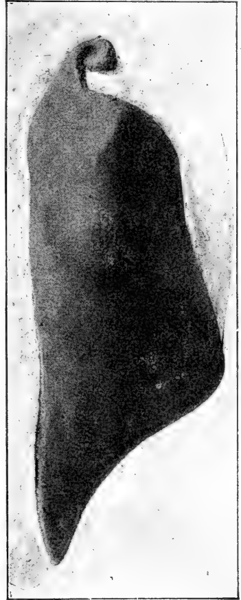
FIG. 11. Sandalodus laevisissimus N. and W. Keokuk limestone, Keokuk, Iowa. Posterior dental plate of left mandibular ramus, \times \frac{2}{3} .
