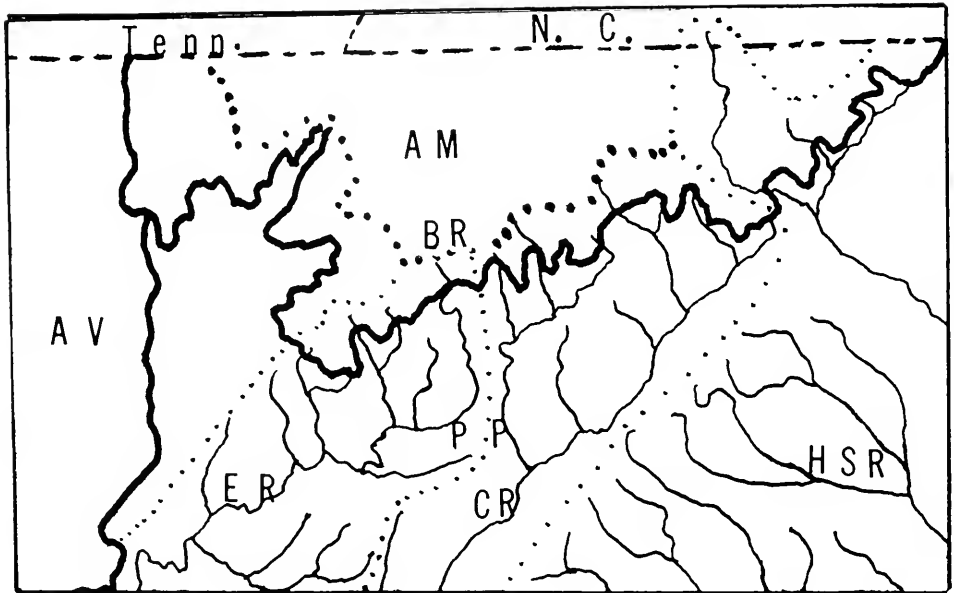
Text-figure 1. Northern Georgia, illustrating the propinquity of the headwaters of the Etowah River (ER), of the Alabama-Caasa; of the Chattahoochee River (CR), of the Apalachicola; and of the Savannah (HSR) river systems. The topographic areas are the Appalachian Mountains (AM), Appalachian Valley (AV), and the Piedmont Plateau (PP). The Blue Ridge divide (BR) is indicated by large dots. The minor divides are indicated by smaller dots. (After Keith, 1925, pl. 29.)
