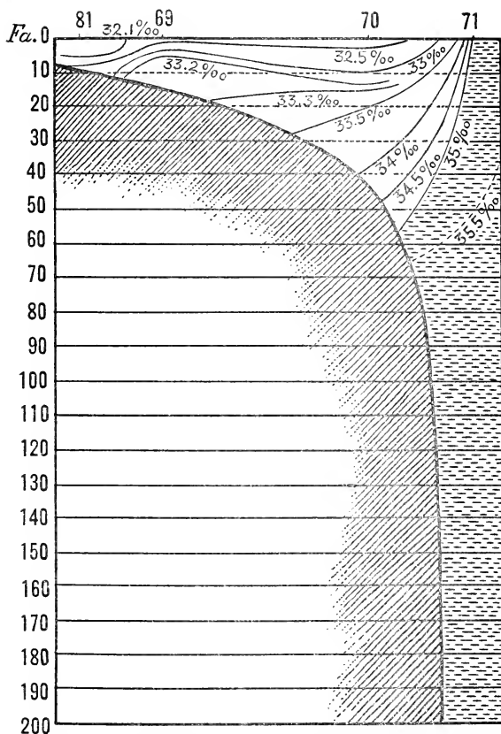
FIG. 40.— Salinity profile across the continental shelf abrest of Barnegat to the edge of the Gulf Stream in Lat. 38^{\circ} 56' (Stations 10081, 10069, 10070, 10071).
