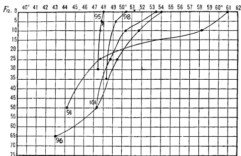
FIG. 19.— Temperature sections in the Gulf of Maine, on Jeffrey's Bank (Station 10091); off Matinicus Island (Station 10101); off the coast of Maine near the Grand Manan Channel (Station 10098); near Lurcher Shoal (Station 10096); and on German Bank (Station 10095).
