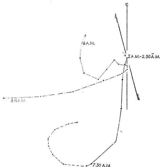
FIG. 65.— Surface current ———, 4 fathom current — · · · — ·, and bottom current . . . ., at Station 10072; hourly from 2 A.M. to 8 A.M., July 21. The surface current of Station 10074, . . . ., is combined with Station 10072 to show total drift for an entire tide. 2.25 cm. = 1 sea mile.
