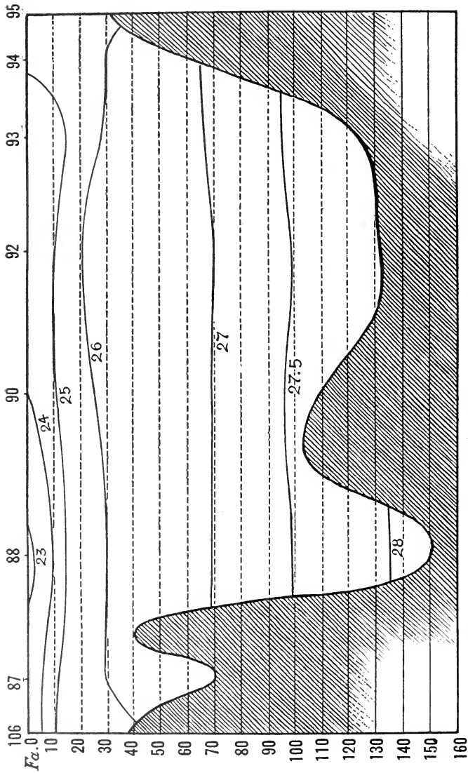
FIG. 62.—Density profile across the Gulf of Maine from Massachusetts Bay to German Bank (Stations 10106, 10087, 10088, 10090, 10092, 10093, 10094, 10095) August 9-20.
