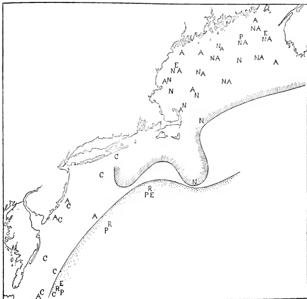
FIG. 69.— Distribution of copepods, July–August, 1913.
