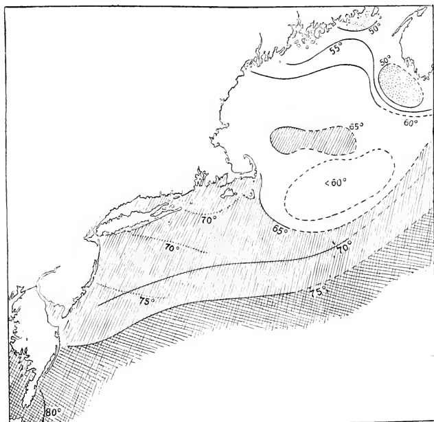
FIG. 1.— Surface temperature for the waters south of Cape Cod in July, and for the Gulf of Maine in August, constructed from the hourly readings. Temperatures below 50^{\circ} , dotted; 65^{\circ} to 75^{\circ} , single hatched; over 75^{\circ} , cross hatched; dotted curves, July 30–Aug. 1, 75^{\circ} , 70^{\circ} .
