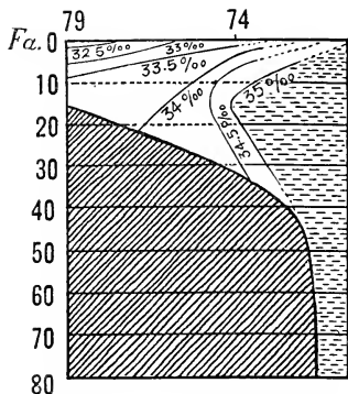
FIG. 41.—Salinity profile across the continental shelf south of Delaware Bay (Stations 10079, 10074).
