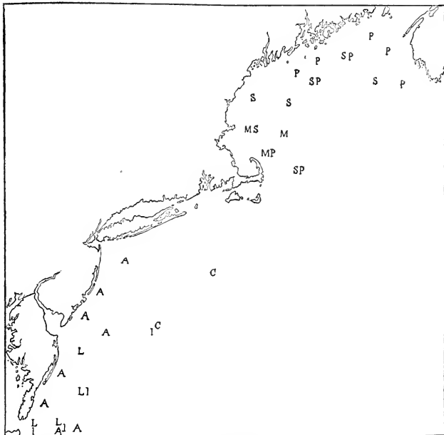
FIG. 79.— Occurrence of some neritic Medusae, July–August, 1913.
