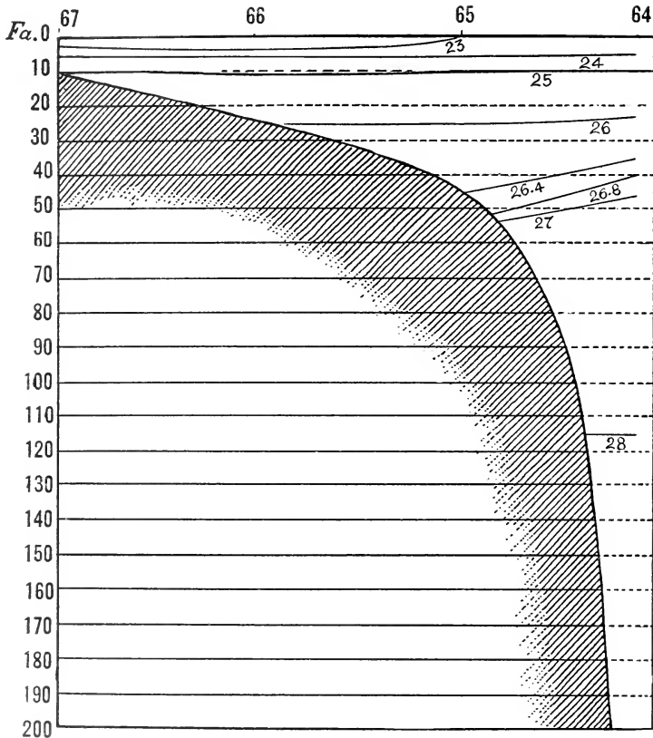
FIG. 58.— Density profile from New York to the edge of the Gulf Stream in Lat. 39^{\circ} 55' (Stations 10067, 10066, 10065, 10064) July 11-13.
