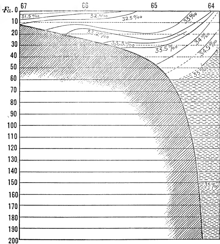
FIG. 39.— Salinity profile across the continental shelf from New York to the edge of the Gulf Stream in Lat. 39^{\circ} 55' (Stations 10067, 10066, 10065, 10064).
