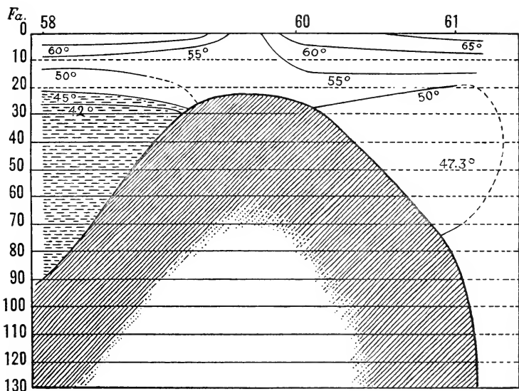
FIG. 9.— Temperature profile from the southern end of the basin of the Gulf of Maine (Station 10058) across Nantucket Shoals to the continental slope south of Nantucket (Station 10061).
