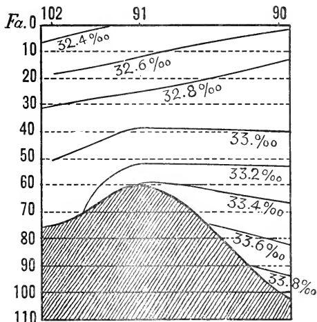
FIG. 50.—Salinity profile from Station 10102, off the mouth of Penobscot Bay, across Jeffrey's Bank (Station 10091) to the centre of the Gulf of Maine (Station 10090).
