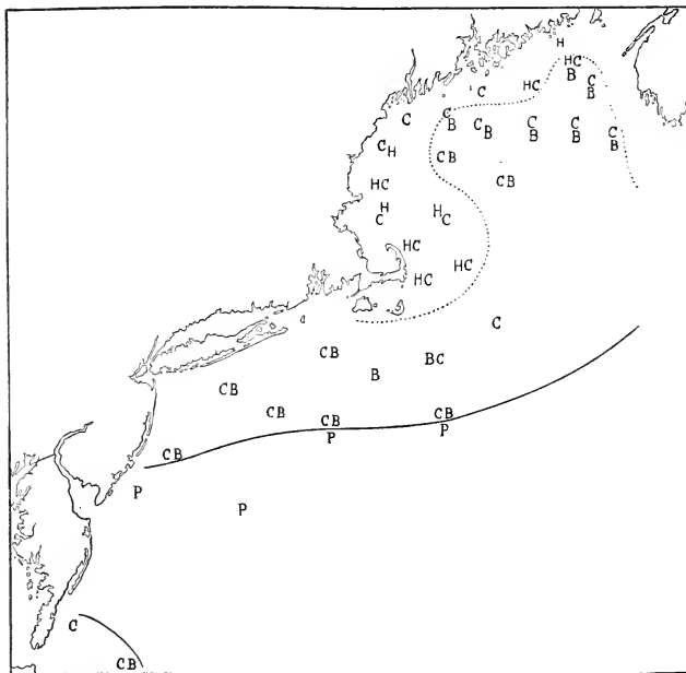
FIG. 68.— Distribution of hyperiid amphipods.
