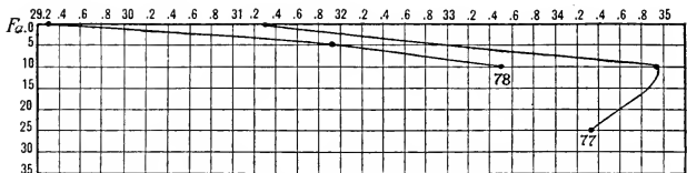
FIG. 34.—Salinity sections on the continental shelf abreast of Chesapeake Bay (Stations 10077, 10078).
