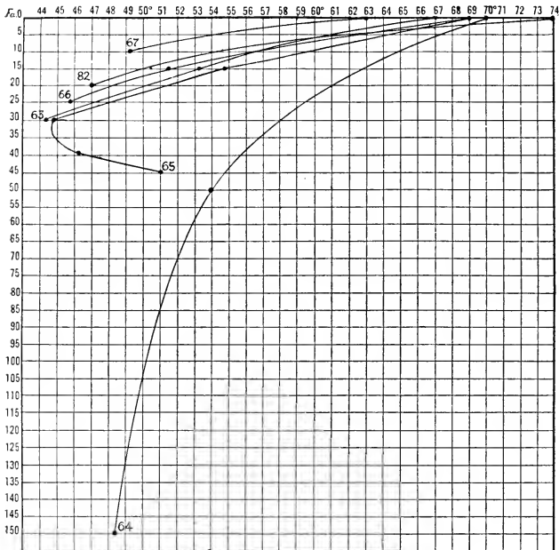
FIG. 4.—Temperature sections on the continental shelf off New York and Long Island (Stations 10063, 10065, 10066, 10067, 100S2) and at the edge of the Gulf Stream, Lat. 39^{\circ} 55' (Station 10064).
