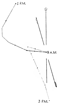
FIG. 64.—Surface current———, and bottom current.....at Station 10065; hourly from 9 A.M. to 3 P.M., July 12. The distance between dots (.) shows the drift for each hour; 2.25 cm. = 1 sea mile. The compass arrows are true and magnetic.
