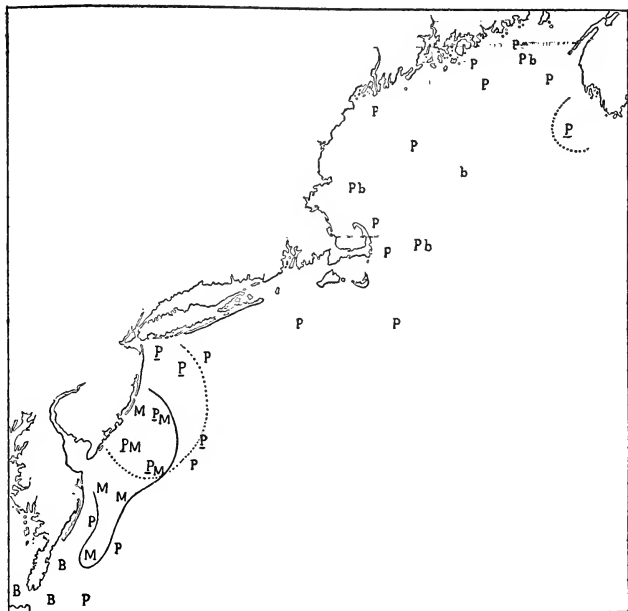
FIG. 80.— Distribution of ctenophores, July–August, 1913.
