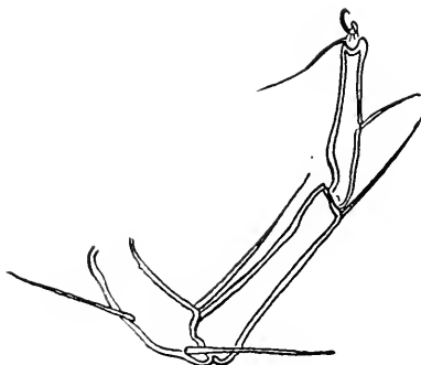
FIG. 5.—Seventh limb.
