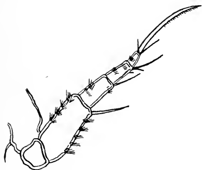
FIG. 4.—Sixth limb.
