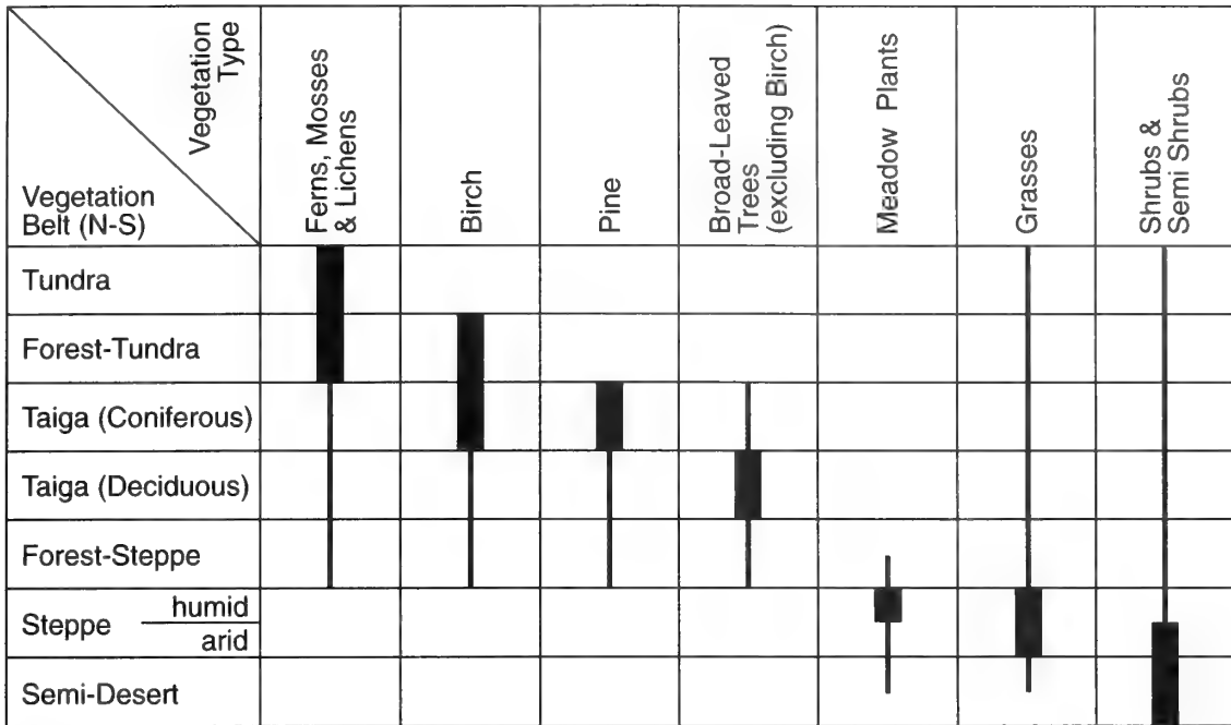
Fig. 3 Distribution of principal vegetation types in relation to vegetation belts. Compiled from various sources. Bar width provides a measure of abundance.
