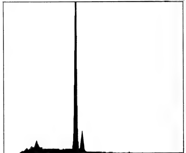
Fig. 9 Plot from qualitative energy dispersive X-Ray microanalysis of non-coated fragments using scanning electron microscopy. The plot displays a major calcium peak (plus a secondary peak to its right), but no phosphorus and only minor amounts of elements with lower atomic weights, to the left.
