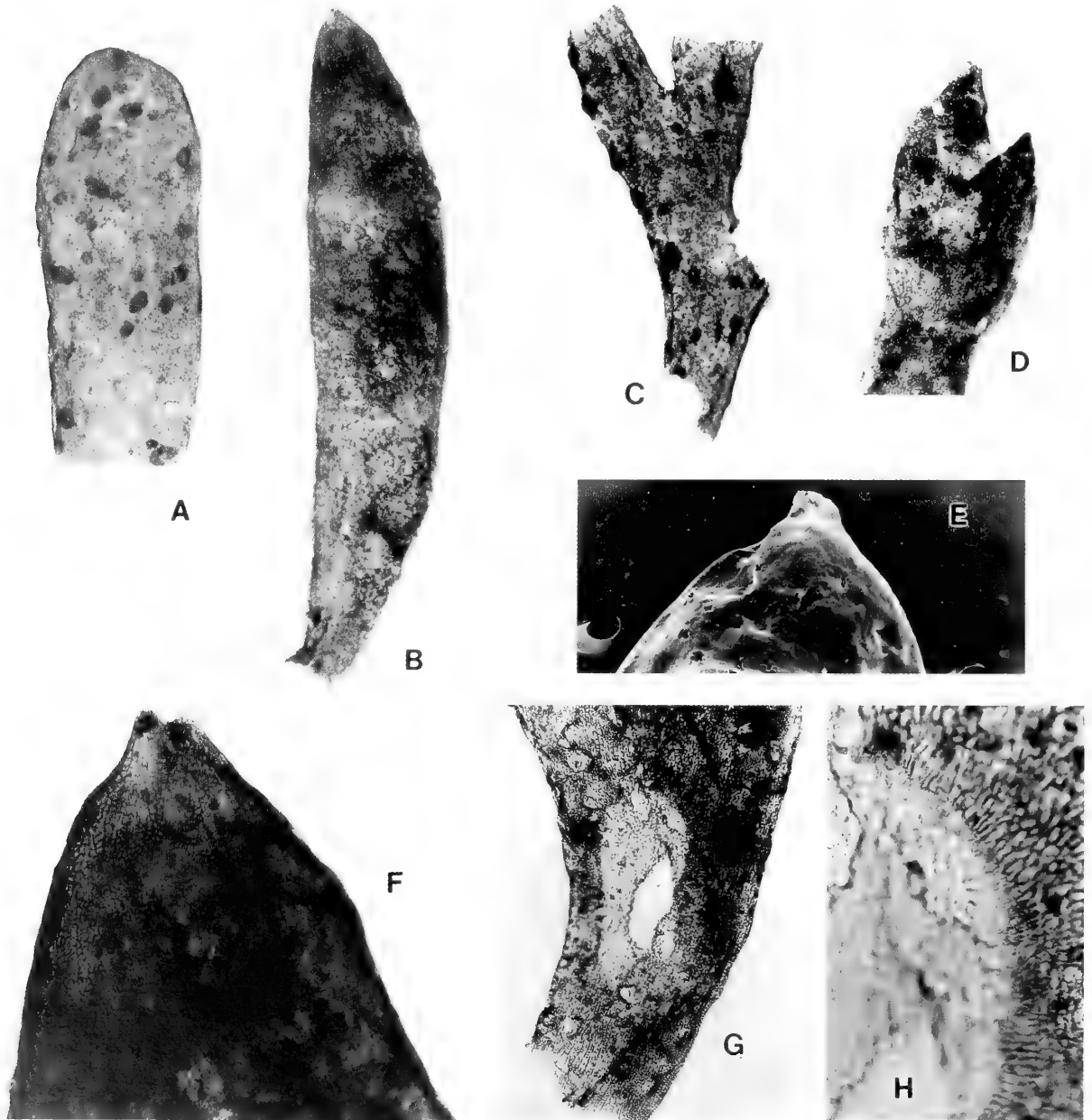
Fig. 7 A–H Ginkgoites weatherwaxiae sp. nov. A , leaf segment with rounded apex and numerous resin bodies, V.64528, LM, \times 15 ; B , large leaf segment with mucronate apex, V.64529, LM, \times 10 ; C , holotype, branched leaf fragment showing two dichotomies, with numerous resin bodies, particularly along left margin, V.64530, LM, \times 10 ; D , forked apex of branched leaf fragment with pointed growing tips, V.64531, LM, \times 20 ; E , unbroken mucronate apex, V.64532, SEM, \times 50 ; F , apex of leaf segment in Fig. B with broken mucronate tip, V.64529, LM, \times 50 ; G , leaf segment showing bite which has pierced both surfaces, V.64533, LM, \times 25 ; H , edge of bite in Fig. G showing evidence of reaction after damage, V.64533, LM, \times 100 .
