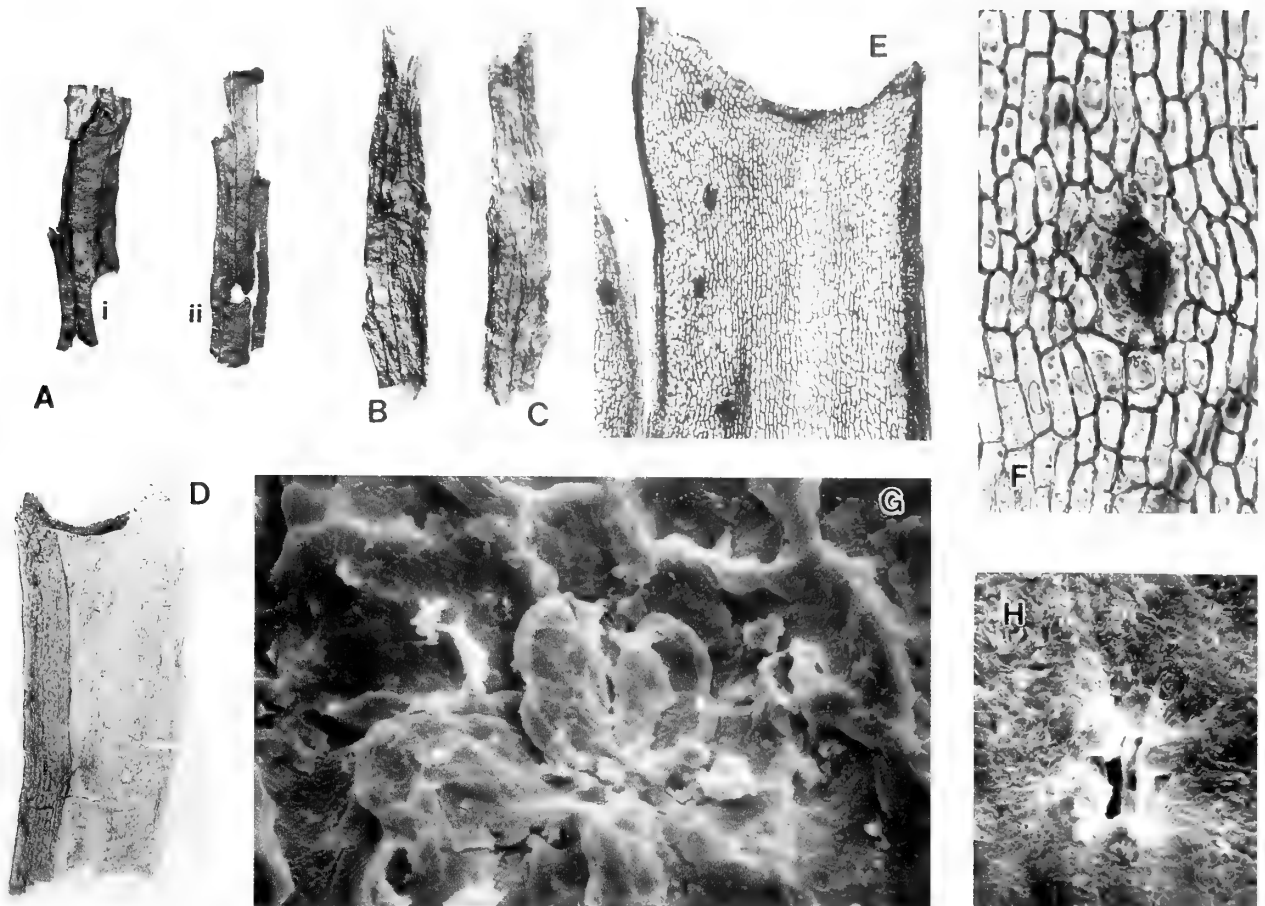
Fig. 31 A–H Sulcatocladus robustus Watson & Harrison. A, B, C , unmacerated shoot fragments showing leaf-scars and decurrent leaf-bases separated by sutures. Ai , V.64256; Aii , V.64257. Wealden, Düingen, North West Germany. \times 2.5 . B, C , two sides of same shoot from English Wealden at Worbarrow Bay, Dorset, V.64589, \times 5 ; D , cuticle of decurrent leaf-base with lower margin of leaf scar at top, V.64590. Galley Hill, East Sussex. \times 25 ; E , cuticle of decurrent leaf-base showing thinner cuticle of longitudinal sutures at each side. Indentation at top is lower part of leaf scar, V.64207, holotype . Wealden; Düingen, North West Germany. LM, \times 60 ; F , stoma on leaf-base cuticle surrounded by epidermal cells with pustules, V.64207, holotype . Wealden; Düingen, North West Germany. LM, \times 125 ; G , stoma viewed from inside showing cutinization of dorsal and ventral walls of guard cells, V.64291. Galley Hill, East Sussex. SEM, \times 750 ; H , outside view of stomatal pit, overhung by subsidiary cell papillae, V.64292, dispersed cuticle from Wealden; Düingen, North West Germany. SEM, \times 750 .
