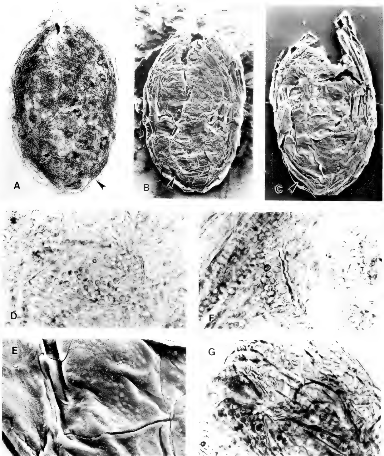
Fig. 20 A–G Ovule attributed to Ginkgoites weatherwaxiae sp. nov. V.64552. A , ovule seen in the light microscope, showing general morphology and two layers of cuticle; arrow indicates gap between them; LM, \times 125 ; B , ovule mounted on a stub with same side uppermost as for LM in A ; outer cuticle present over most of the surface; where absent, showing well-defined wall dividing inner cuticle, SEM, \times 125 ; C , ovule remounted to show reverse side; outer cuticle present only at margins, inner cuticle showing polygonal cells divided by cracks; arrow indicates gap between them; SEM, \times 125 ; D , inner cuticle showing aggregation of vesicles in centre of cell, LM, \times 750 ; E , inner cuticle showing cracks defining cell margins and raised impressions of vesicles, SEM, \times 750 ; F , well-defined wall seen in middle of apical end of inner cuticle, LM, \times 750 ; G , two pollen grains found in outer cuticle in apical region, LM, \times 750 .
