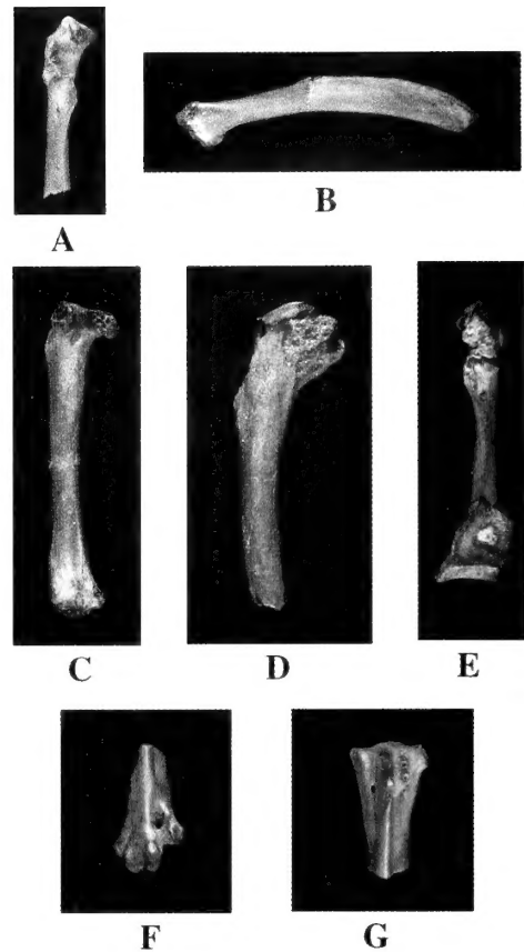
Fig. 2 Pseudasturid specimens from the London Clay Formation. A–E , BMNH A 6218; A , portion of left coracoid; B , left scapula; C , left femur; D , portion of right humerus; E , right coracoid. F , BMNH A 6184, distal end of a left tarsometatarsus. G , BMNH A 6224, proximal right tarsometatarsus. All figures are \times 2 .
