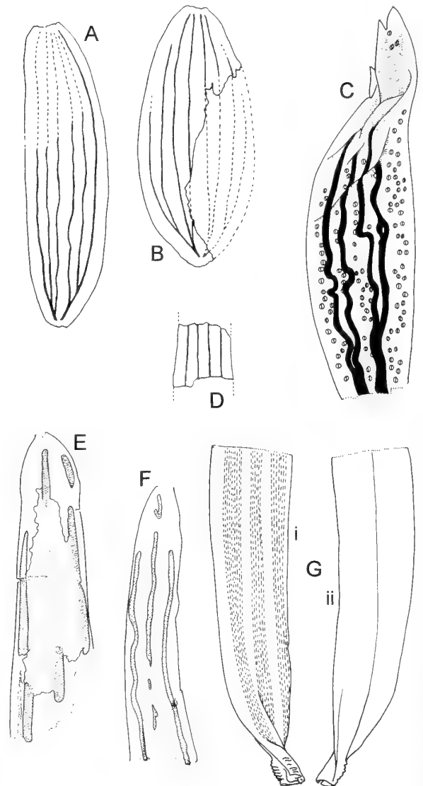
Fig. 23 A–G Pseudotorellia linkii (Römer) Watson & Harrison. A, B , wide elliptical leaves from the English Wealden. A , V.51525; B , V.51528; C , leaf showing two dichotomising veins and positions of stomata, V.64243, \times 15 ; D , part of sub-parallel-sided leaf with 4 veins, V.51527; A, B, D after Watson 1969, all \times 10 ; E , distal part of leaf with 3 resin canals, V.64239, \times 10 ; F , distal leaf fragment with 3 resin canals, V.64240, \times 10 ; G , leaf with twisted, wrinkled base; i , lower surface showing position of 3 stomatal bands; ii , upper surface with grooving midline, V.64250, \times 6 .
