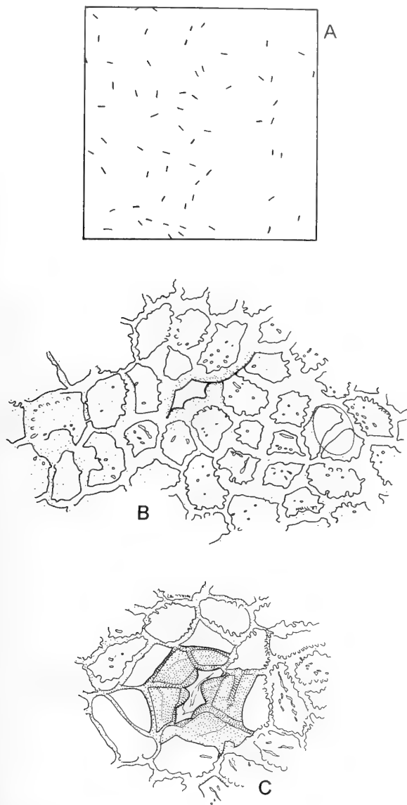
Fig. 13A–C Ginkgoites nannoygiae sp. nov. All show holotype, V.64545, from Fairlight Clays of the Ashdown Beds, Galley Hill, Sussex. A , stomatal distribution for lower cuticle, \times 50 ; B , upper cuticle showing pitting of anticlinal and outer periclinal walls of epidermal cells, a stoma (left hand side) with ill-defined subsidiary cells and an oval scar overlying two epidermal cells, \times 400 ; C , a single stoma (right hand side) giving darker appearance; outline of guard-cell dorsal plates unclear in places, \times 400 .
