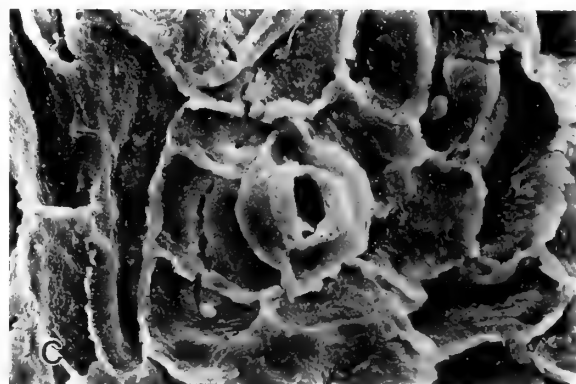
Fig. 18 A–C Ginkgoites garlickianus sp. nov. All upper cuticle.
