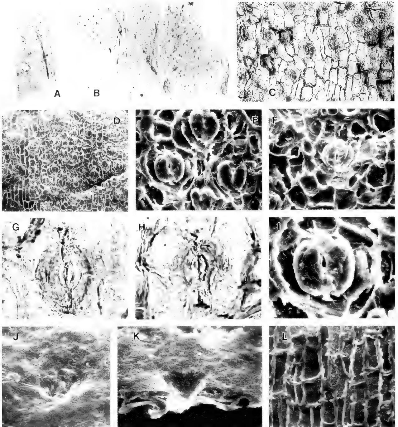
Fig. 24 A–I Pseudotorellia vimesiana sp. nov. A , apical portion of leaf with tip missing. LM, V.64554, \times 25 ; B , holotype : leaf fragment opened up to show stomata confined to one surface (?lower). V.64555, \times 25 ; C–L , all from V.64556: C , lower cuticle with stomata. LM, \times 125 ; D , inside surface of lower cuticle showing stomata arranged in three indistinct bands. SEM, \times 75 ; E , four stomata viewed from the inside. SEM, \times 250 ; F , single stoma viewed from the inside surrounded by rings of subsidiary and encircling cells. SEM, \times 250 ; G , H , stomata showing oval rim to pit (in top plane of focus) and polar appendages to guard cells (in lower plane of focus). LM, \times 500 ; I , stoma viewed from the inside with distinct cutinization of ventral as well as dorsal periclinal walls of guard cells. SEM, \times 500 ; J , crater-like stomatal pit. SEM, \times 500 ; K , cut section through a stomatal pit. SEM, \times 500 ; L , inside surface of upper cuticle showing outlines of rectangular cells and longitudinal bars. SEM, \times 250 .
