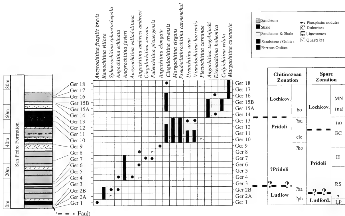
Fig. 10 Selected chitinozoan distribution at Geras. Chitinozoan zonation after Verniers et al. (1995): bo : bohémica, su : superba, ele : elegans, ko : kosovensis, ba : barrandei, ph : philipi.
