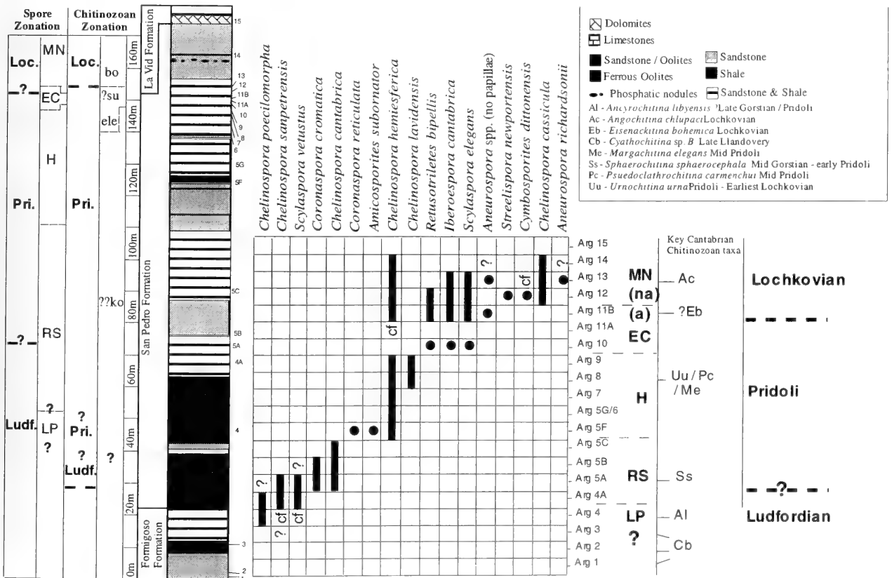
Fig. 3 Selected spore distribution at Argovejo. Chitinozoan zonation after Verniers et al. (1995): bo : bohemia, su : superba, ele : elegans, ko : kosovensis.
