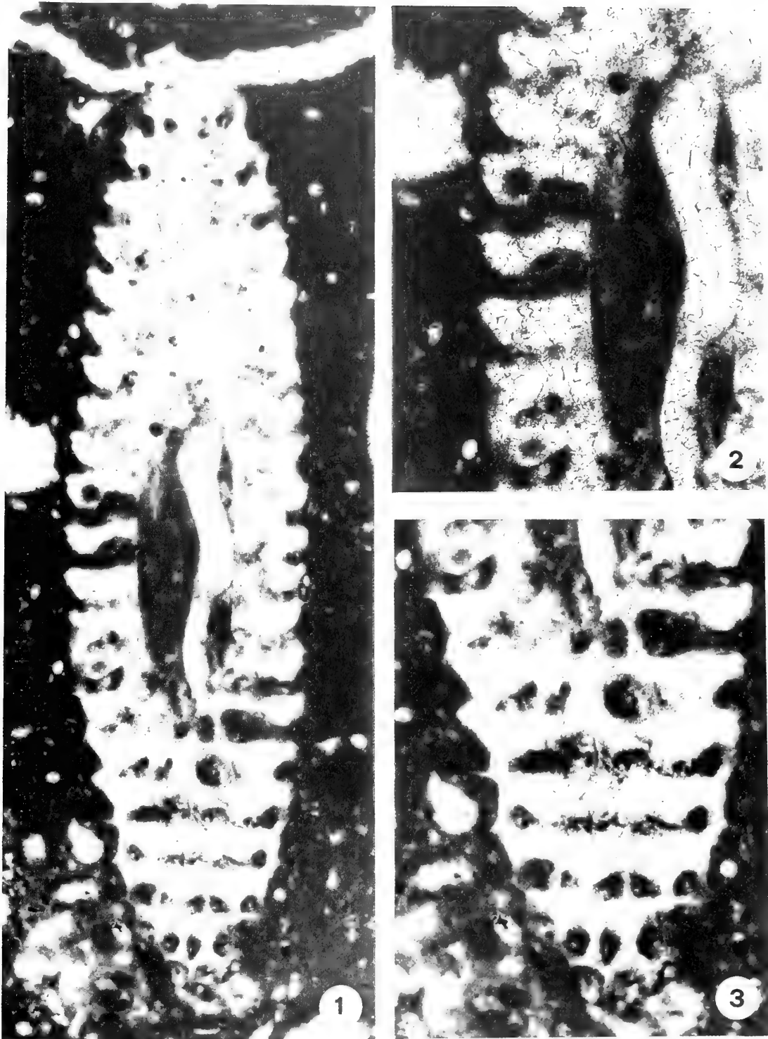
Fig. 1 Neomeris (Larvaria) assurbanipali Elliott nov. comb. Oblique section. Lower Cretaceous (Valanginian – Hauterivian). Garagu formation, Erbil Liwa, Iran; V.52032, \times 34 .
