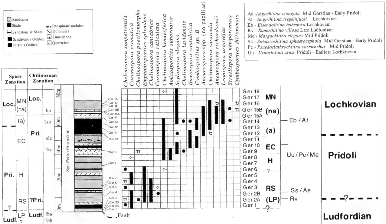
Fig. 2 Selected spore distribution at Geras. Chitinozoan zonation after Verniers et al. (1995): bo : bohemia, su : superba, ele : elegans, ko : kosovens, ba : barrandei, ph : philipi.
