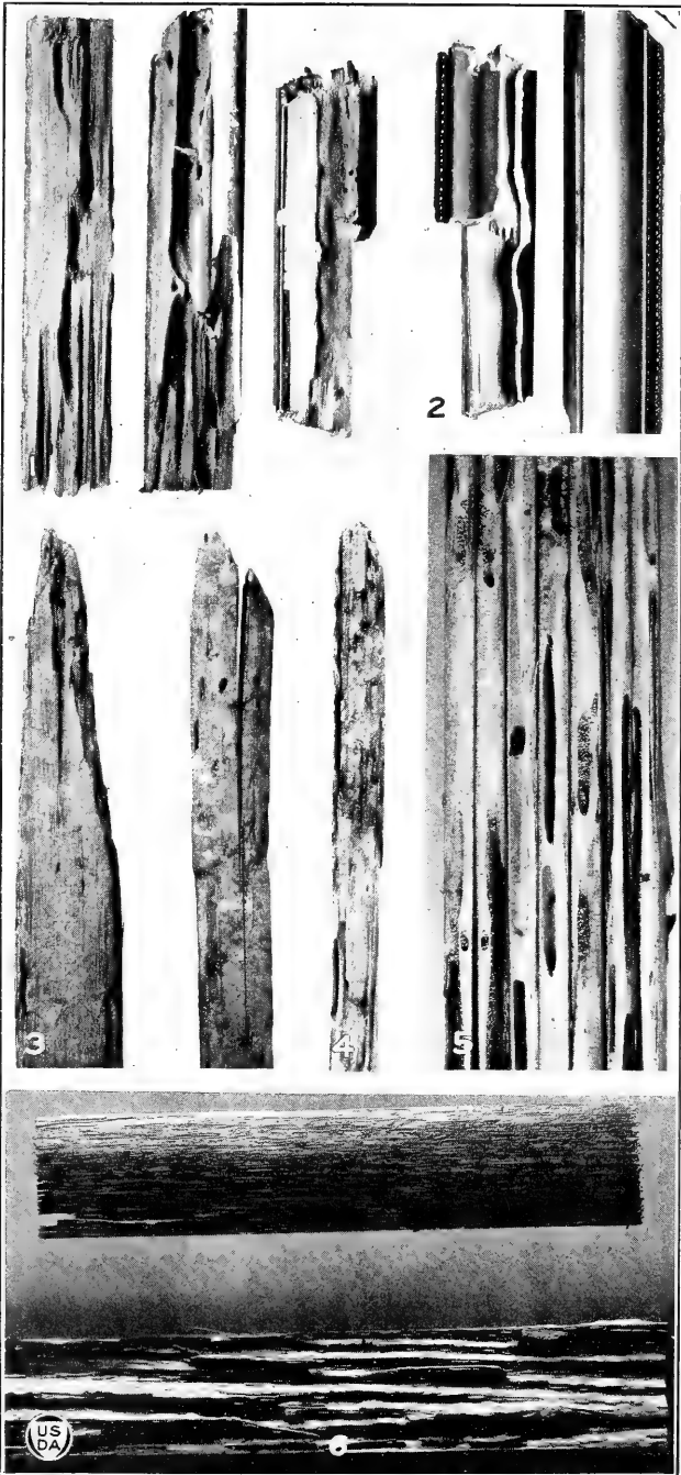
RESISTANT REDWOOD DAMAGED BY NATIVE TERMITES, AND OTHER DAMAGE TO WOOD BY TERMITES.
