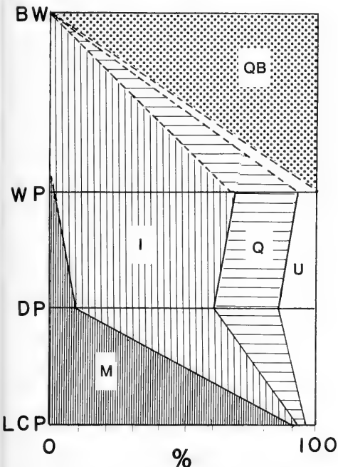
Text-figure 13.—Proportional representation of the four Bulliopsis morphotypes at each of the four stratigraphic levels sampled in the Chesapeake Bay region. Vertical axis is stratigraphic order; horizontal axis is percent of all Bulliopsis found at that level. BW = Bowler's Wharf, loc. 6; WP = Windmill Point, loc. 3; DP = Deep Point, loc. 5; LCP = Little Cove Point, loc. 1; M = marylandica ; I = integra ; Q = quadrata ; QB = quadrata bowlerensis ; U = unidentified. Figure is based on data from only the four sampled levels, and data points representing these localities are connected by straight lines; actual abundances between these levels are unknown.
