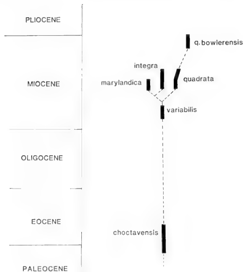
Text-figure 19.—Summary phylogenetic tree for all species of Bullia ( Bullioopsis ). Solid lines represent known stratigraphic ranges of species and subspecies; dashed lines represent inferred phylogenetic relationships.
