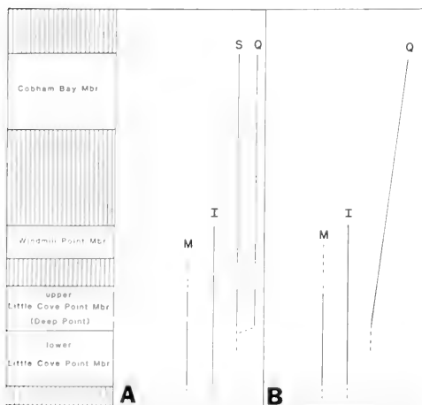
Text-figure 8.—Alternative scenarios for the evolution of Miocene species of Bullioipsis . A , Bullioipsis subquadrata [S] and Bullioipsis quadrata [Q] are separate species differing in degree of sculpturing, and both persist into the Cobham Bay Member of the Eastover Formation. B , All post-St. Mary's Bullioipsis belong to a single, variable species, Bullioipsis quadrata , [Q], which originated in lower or middle St. Mary's time and became increasingly sculptured. M = Bullioipsis marylandica ; I = Bullioipsis integra . Dashed lines indicate undetermined points of origin and/or extinction.
