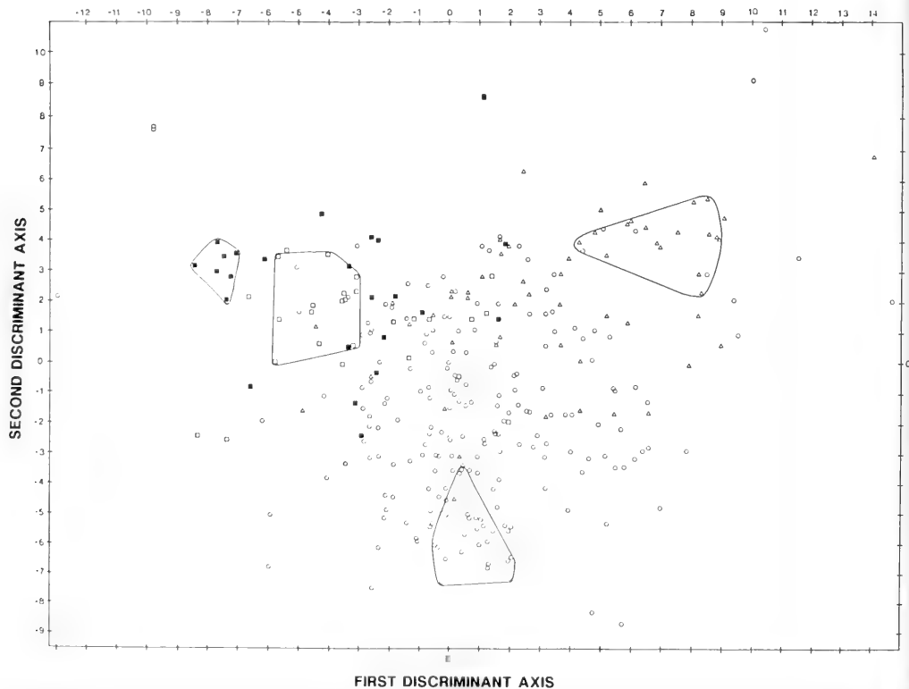
Text-figure 12.—Scatterplot of scores on the first two discriminant axes for all specimens of Bullioopsis collected from the Chesapeake Bay region for this study. The four select groups are outlined, \Delta = integrata (total group 1); \circ = marylandica (total group 2); \square = quadrata + subcylindrica from Maryland St. Mary's (total group 3); \blacksquare = Bowler's Wharf specimens (total group 4).
