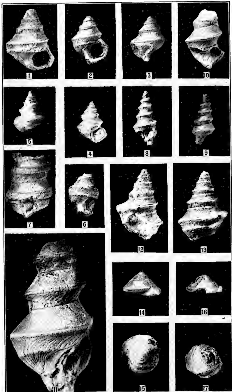
KANGYAO FORMATION
