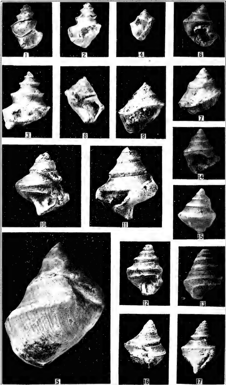
KANGYAO FORMATION
