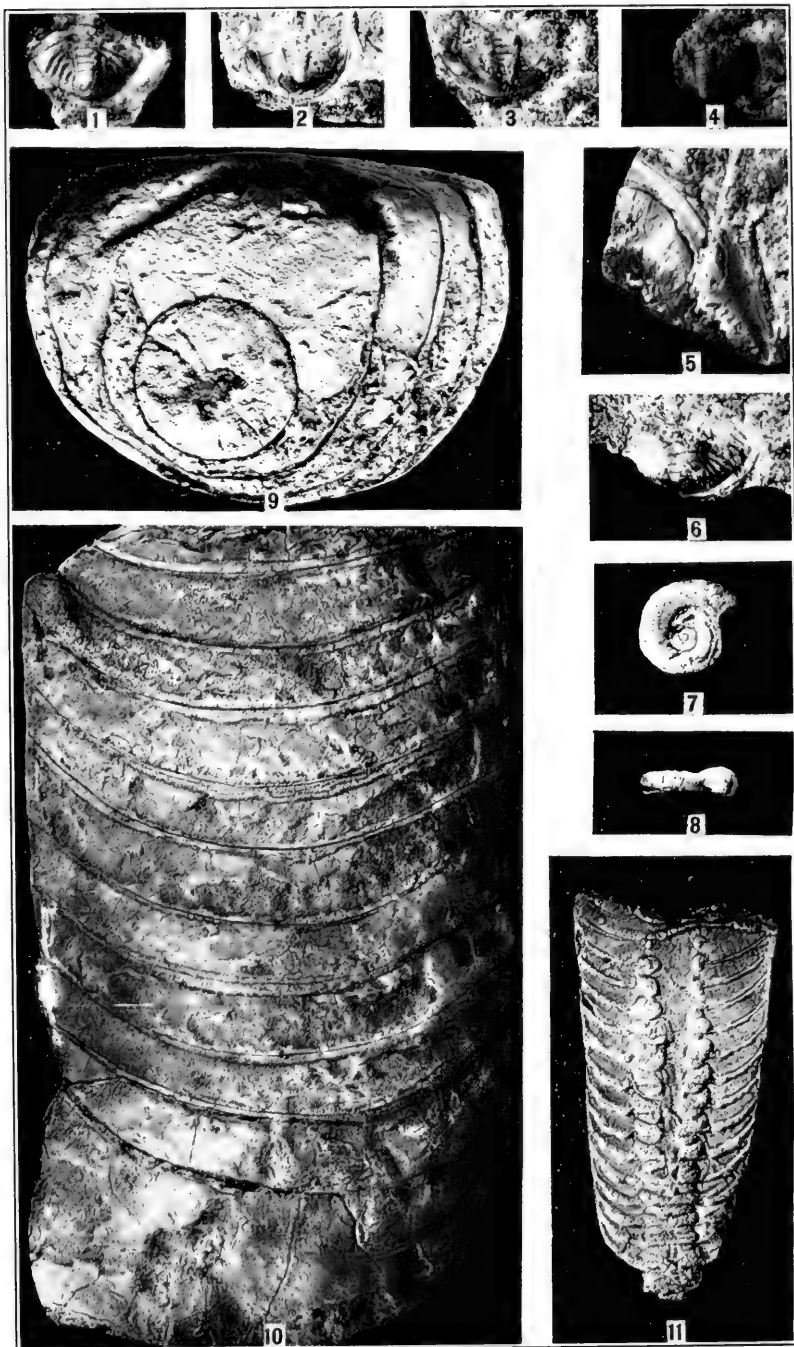
WUTING FORMATION
