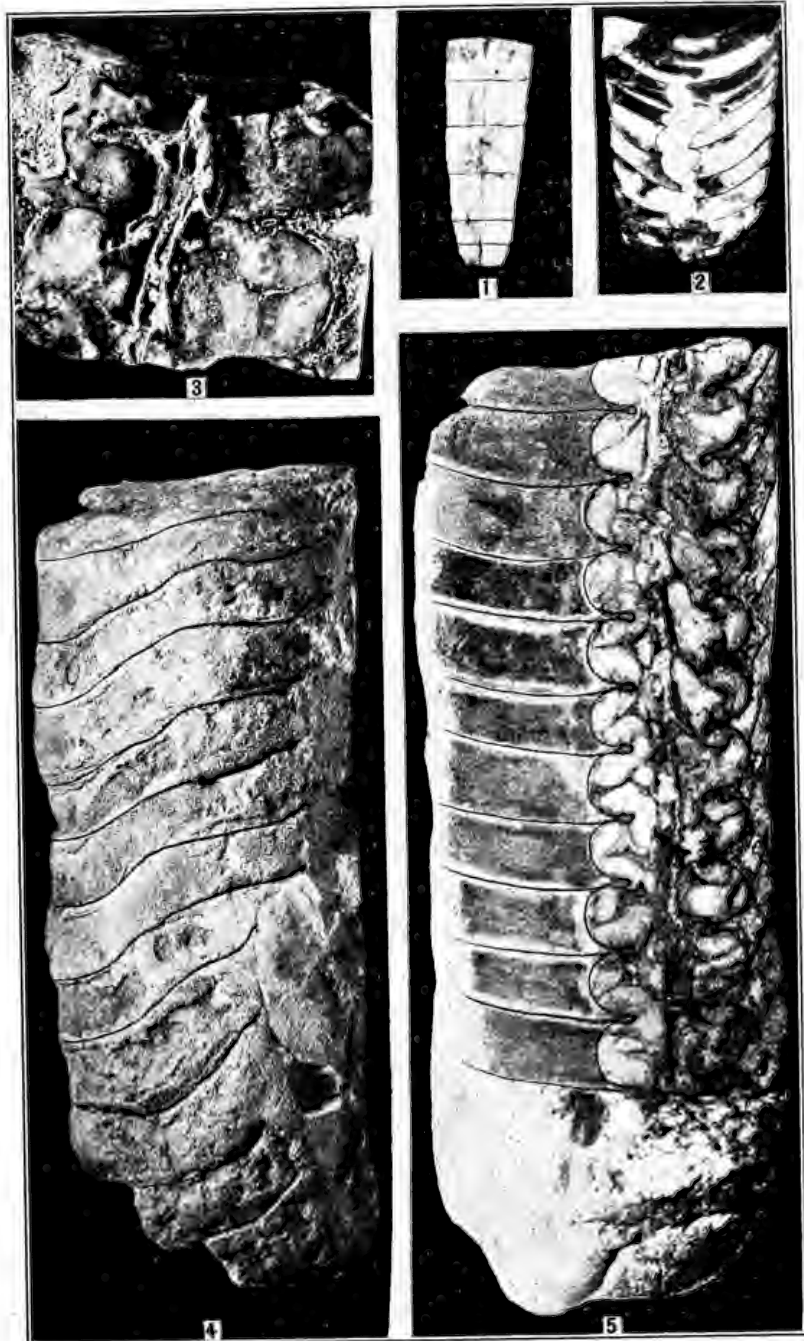
WUTING FORMATION
