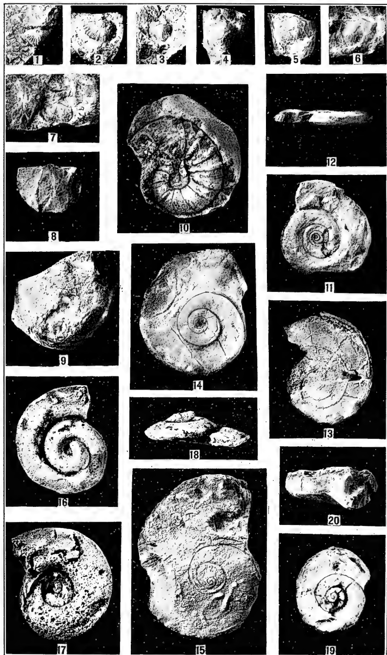
WUTING FORMATION
