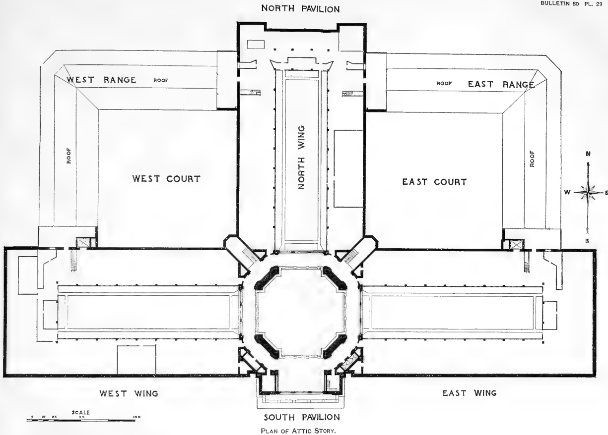
PLAN OF ATTIC STORY.
