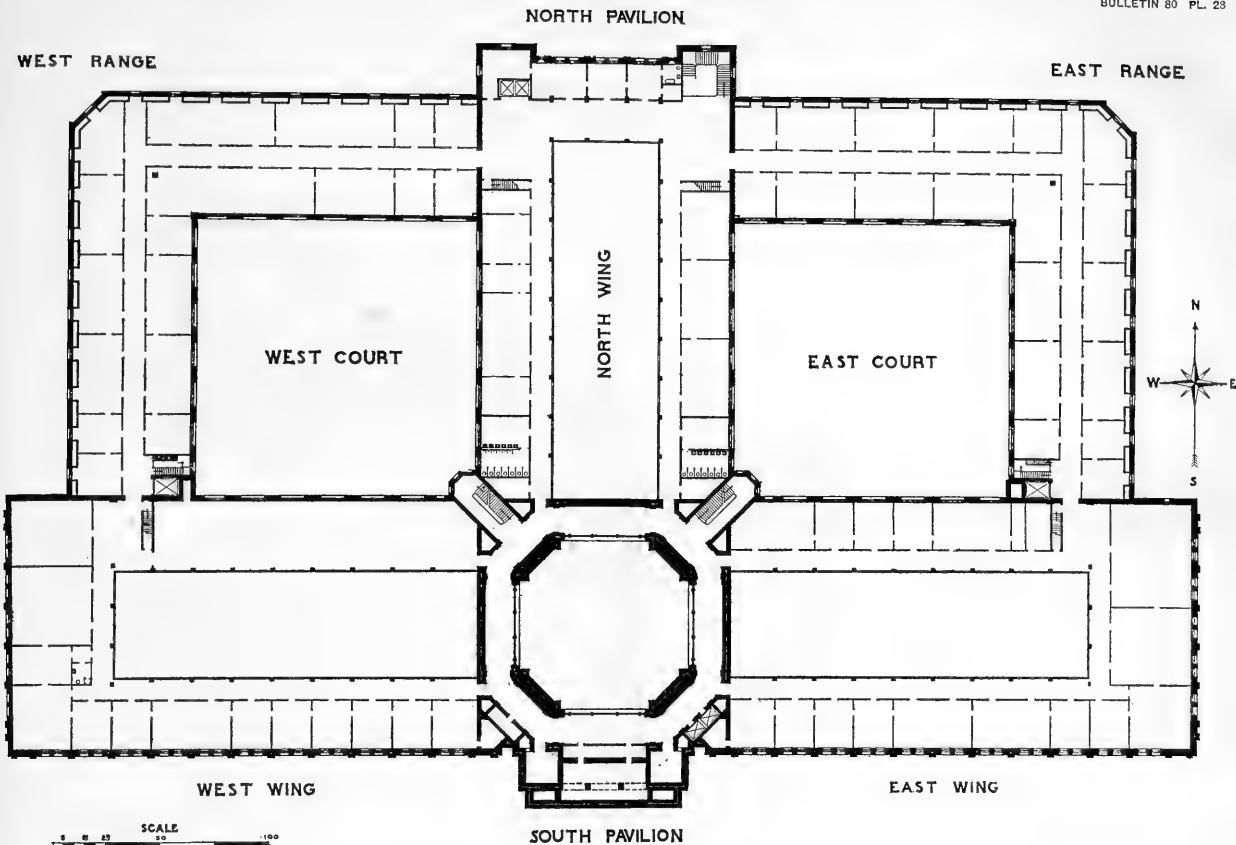
PLAN OF THIRD STORY.
