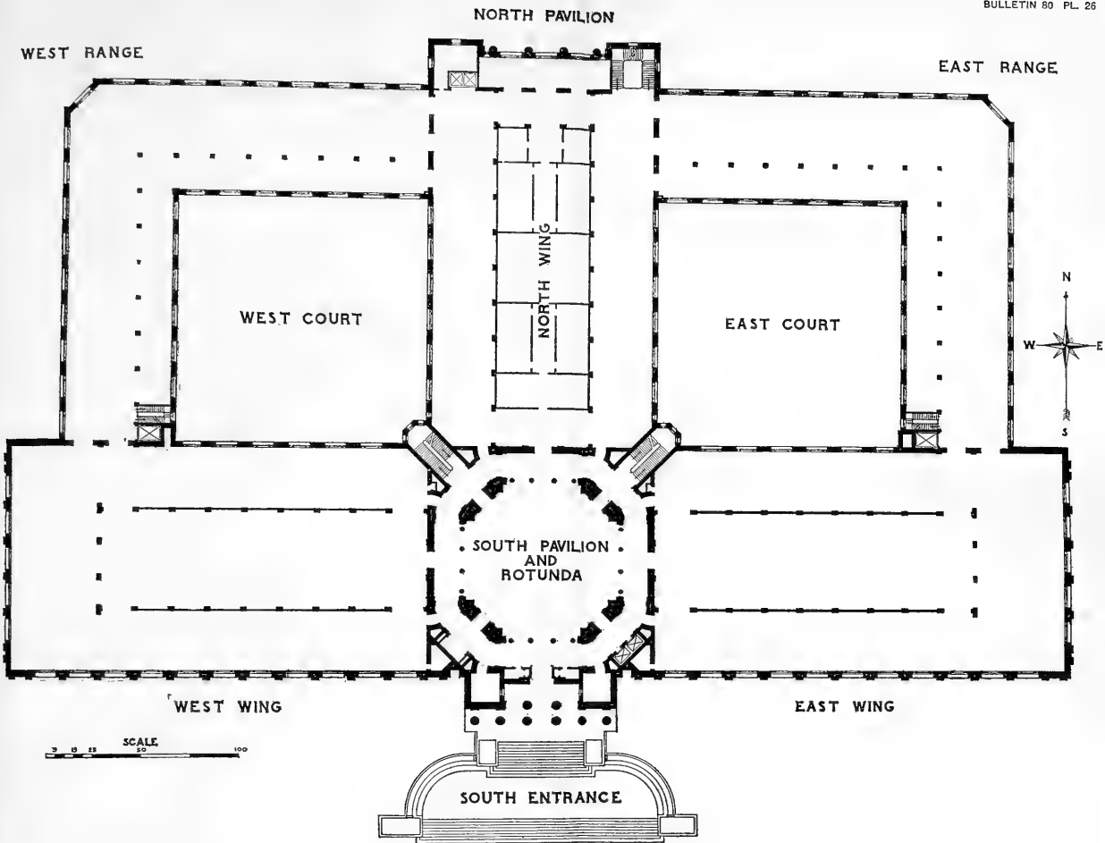
PLAN OF FIRST STORY.
