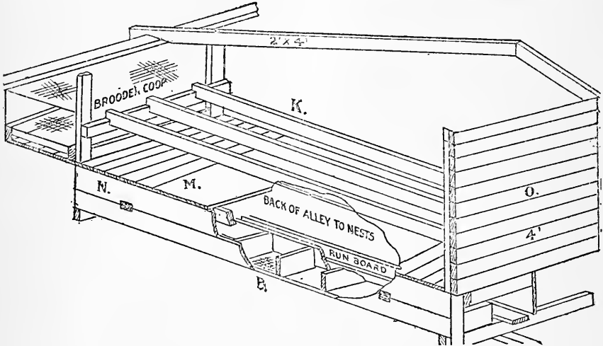
DETAILS OF ROOST AND NEST. FIG. 25.
