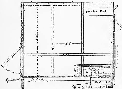
SIDE VIEW BROODER-HOUSE. FIG. 8. SECTIONAL VIEW. FIG. 9.
