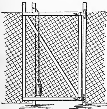
GATE CLOSED. FIG. 35.
