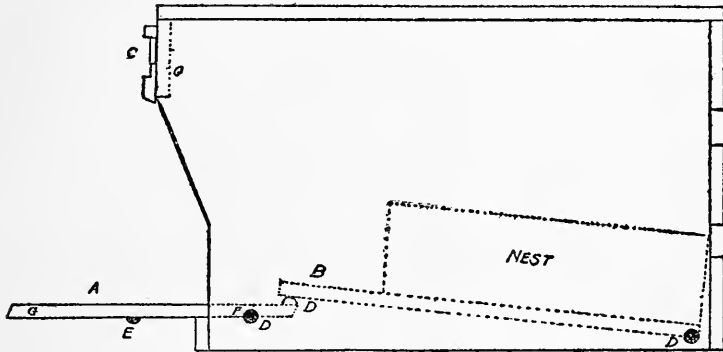
TRAP NEST OPEN. FIG. 48.
