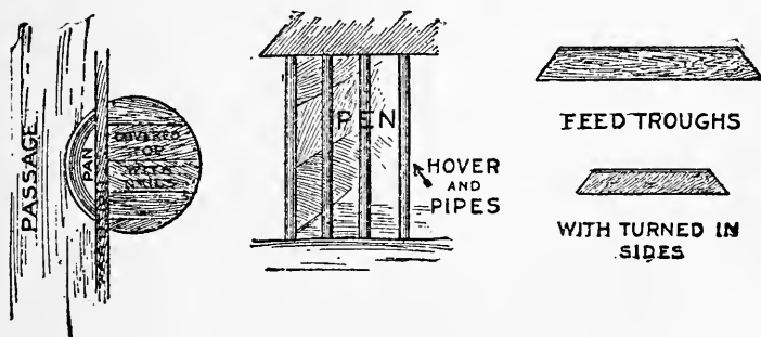
SECTION OF HOUSE INTERIOR. FIG. 51.
