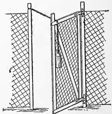
GATE OPEN. FIG. 36.
