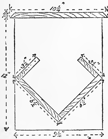
SECTION OF BURR TROUGH. FIG. 53.
