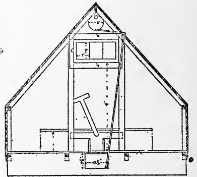
SIDE VIEW BROODER-HOUSE. FIG. 8. SECTIONAL VIEW. FIG. 9.
