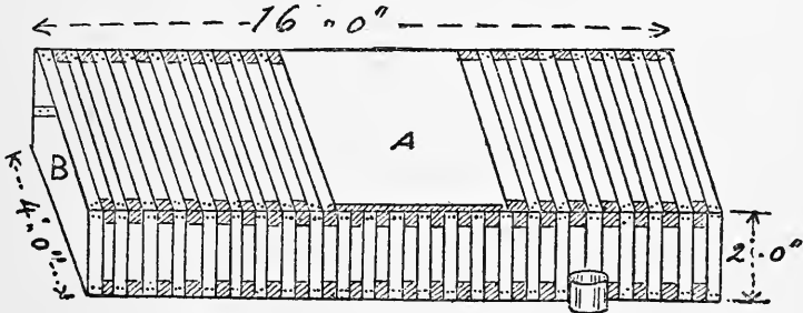
MOVABLE POULTRY YARD. FIG. 50.
