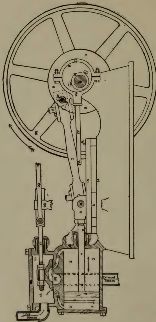
Fig. 5. Steam Engine.
