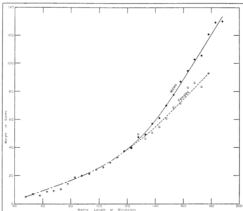
FIGURE 150. Weight-length relationship
