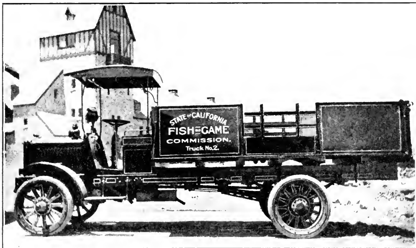
Fig 111. Truck No. 2 at Mt. Whitney Hatchery. By means of two trucks such as this the output of the Mt. Whitney Hatchery is hauled to the railroad station. Photograph by A. E. Culver, 1918.
