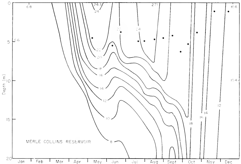
FIGURE 2. Typical Merle Collins Reservoir annual isotherms and Secchi depths (·) from 1966 observations.
