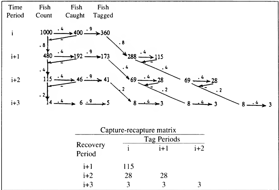
Figure 1. Simulated capture-recapture data matrix for one cohort of carcasses.
