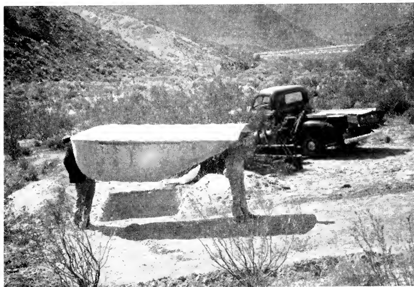
FIGURE 4. Installing one of the new type plastic gallinaceous guzzlers
