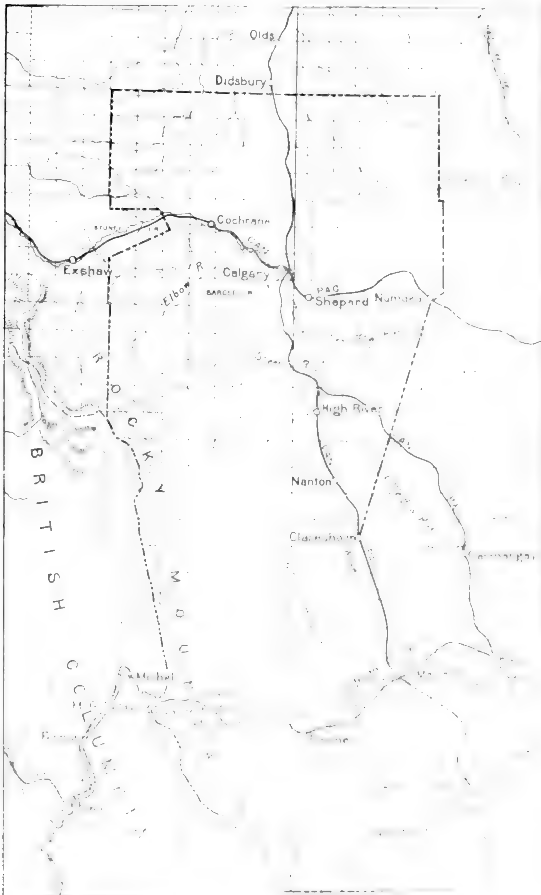
Map of the High River District, Alberta.
