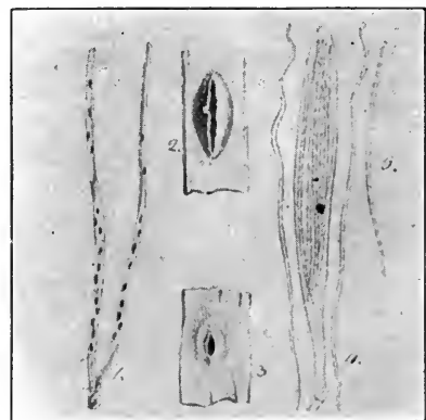
Fig. 1781. Lophodermium pinastri (Pine Leaf Cast). (1) leaves with the fungus. Within the apothecia are the club-shaped asci which contain the spores. (After Masseur).
