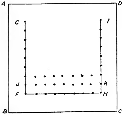
FIG 6. STAKING OUT
