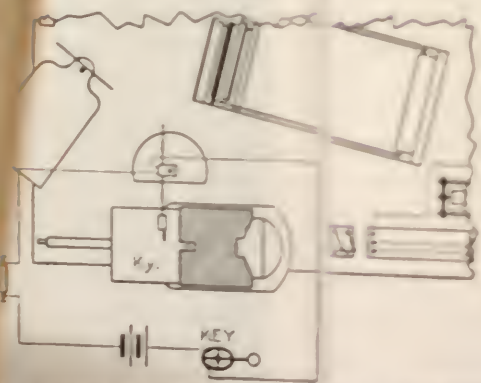
26.—Diagram of the connections for memory experiment.
