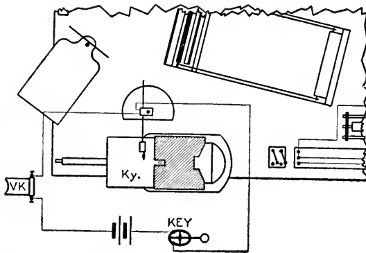
FIG. 26.—Diagram of the connections for memory experiment.
