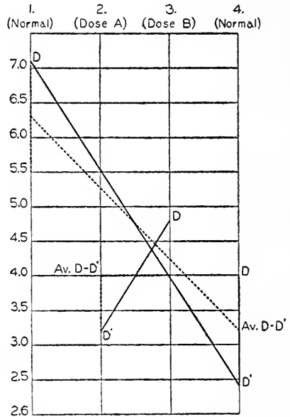
FIG. 25.—Curves of the usualness of the association.
