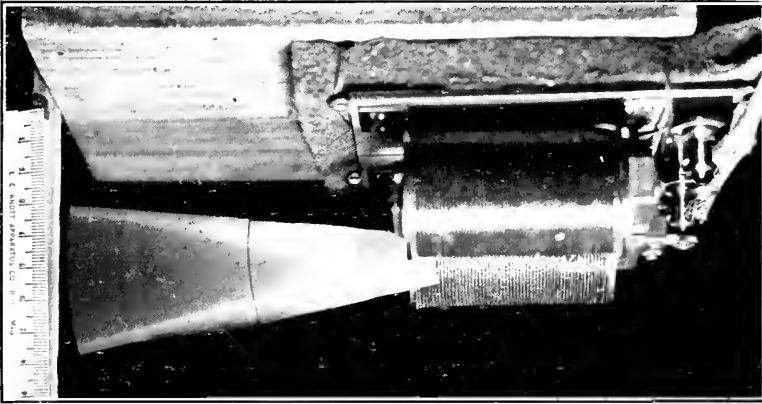
Fig. 7.—Time-recording interruptor at rest.
