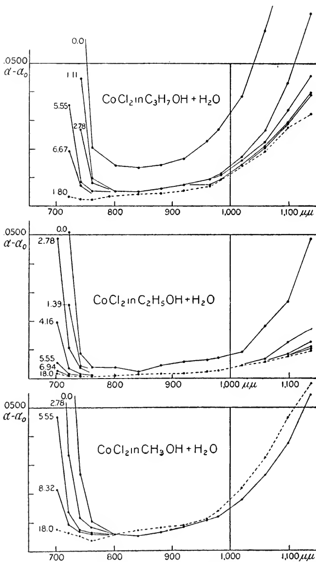
—Curves showing the Differences in Absorption between Solvent and Solutions for Cobalt Chloride in Mixtures of the Alcohols with Water.
