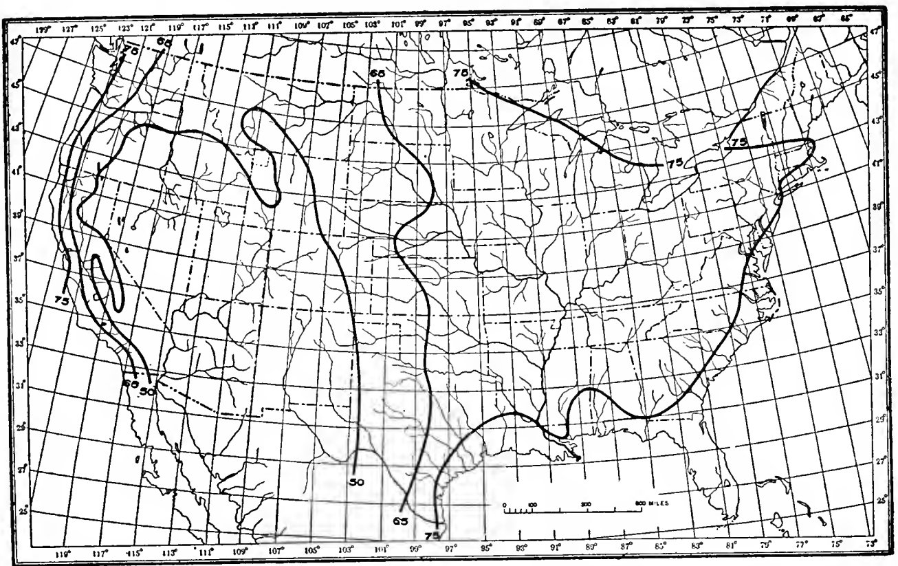
FIG. 17.—Moisture zonation, according to indices of relative humidity for period of average frost-free season. Humidity provinces: Humid , more than 75; semihumid , 65 to 75; semiarid , 50 to 65; arid , less than 50. Numerical values represent percentages. (See also Plate 65.)
