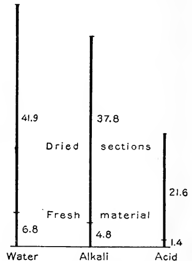
FIG. 17.—Swelling reactions of fresh and dried flower-stalks of Rudbeckia , in percentages of original thickness. The proportionate increase of dried sections is denoted by the heights of the vertical lines, and that of fresh sections by the marks near base.
