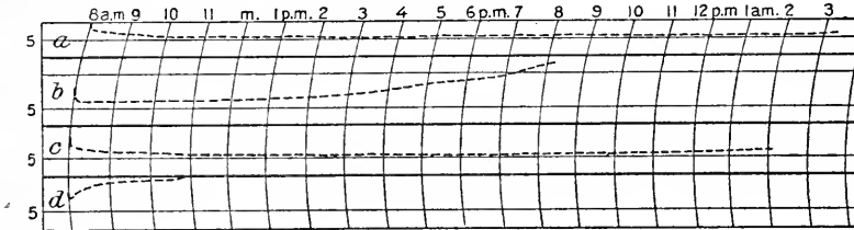
FIG. 18.—Swelling of tangential slices from tips of asparagus shoots at 14° to 17° C., X 20, on scale ruled to 5 mm. and 1-hour intervals. a , swelling of trio 3.8 mm. in thickness 7 per cent in water; b , swelling of trio 3.7 mm. in thickness 4 per cent in hundredth-normal citric acid; complete within a few minutes, followed by gradual shrinkage; c , swelling of trio of sections 6.2 per cent in sodium hydroxid with final shrinkage; d , slight swelling of trio of sections in hundredth-normal potassium chloride and hydrochloric acid and then rapid shrinkage.
