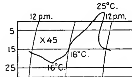
FIG. 34.—Upper part of figure is an auxographic record of variations in thickness of leaf of Mesembryanthemum on a cloudy day with but little change in temperature, as taken by a mercurial thermometer from a similar leaf. Upward course of line denotes increase. \times 45 . Lower figure is an auxographic tracing of same leaf on sunny day with temperatures of 16° to 25° C. Shrinkage occurred during the entire daylight period. \times 45 .
