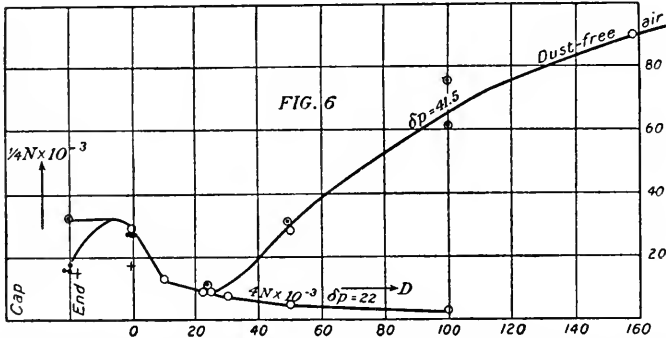
FIG. 6.—Efficient nucleation ( N ) near the middle of the fog chamber, for different distances ( D ) of radium from the end and for different exhaustions ( \delta p ). Table 4.
