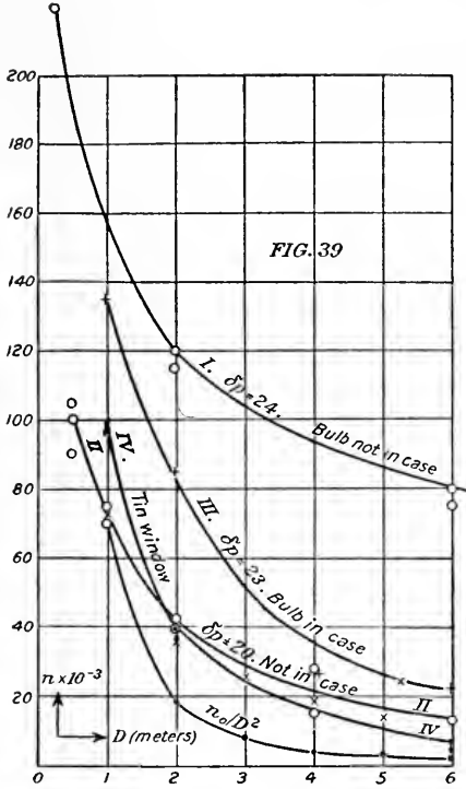
FIG. 39.—Nucleation (ions) produced by a radiating X-ray bulb (cased in lead or not as stated), at different distances ( D ) from the glass fog chamber. Table 32.
