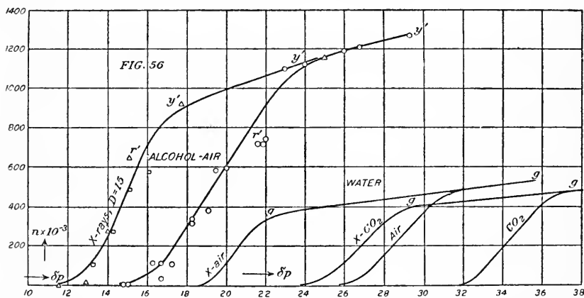
FIG. 56.—Efficient nucleation n in energized or non-energized media of alcohol-air and water-air, at different exhaustions ( \delta p ). Table 46.
