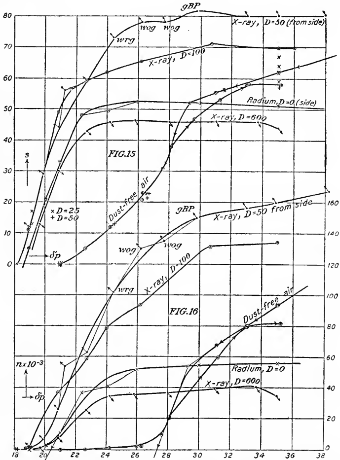
FIGS. 15 and 16.—Early data of efficient nucleations ( N, n ) and coronal diameter ( s ), appearing at different exhaustions ( \delta p ) in dust-free air. Imperfect fog chamber. (Illustrating table 7.)
