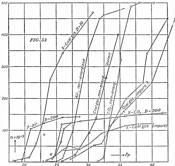
FIG. 53.—Efficient nucleation ( n ) observed in media water-air, water- CO_2 , water-coal gas, energized or non-energized at different exhaustions \delta p .
