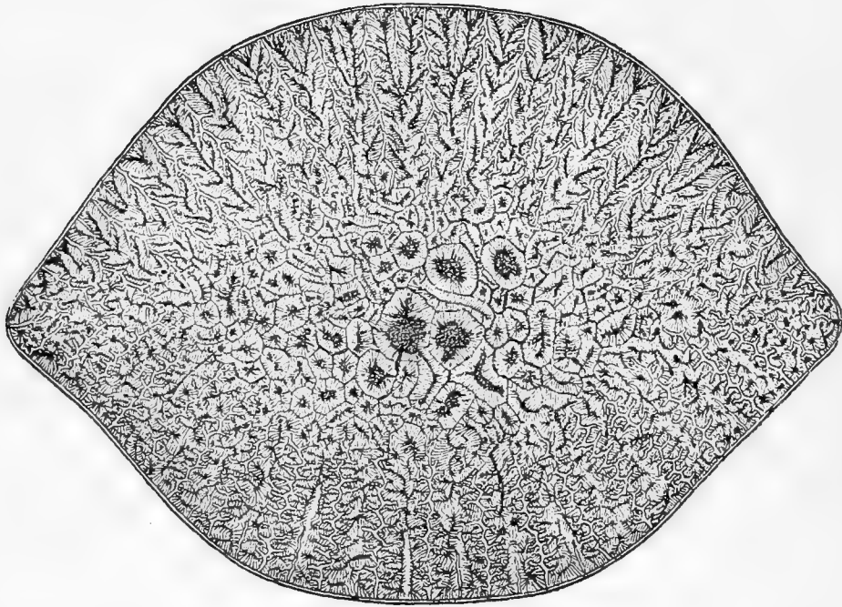
Transverse section of Holoptychian (Dendrodont) Tooth, much magnified; after Pander.
