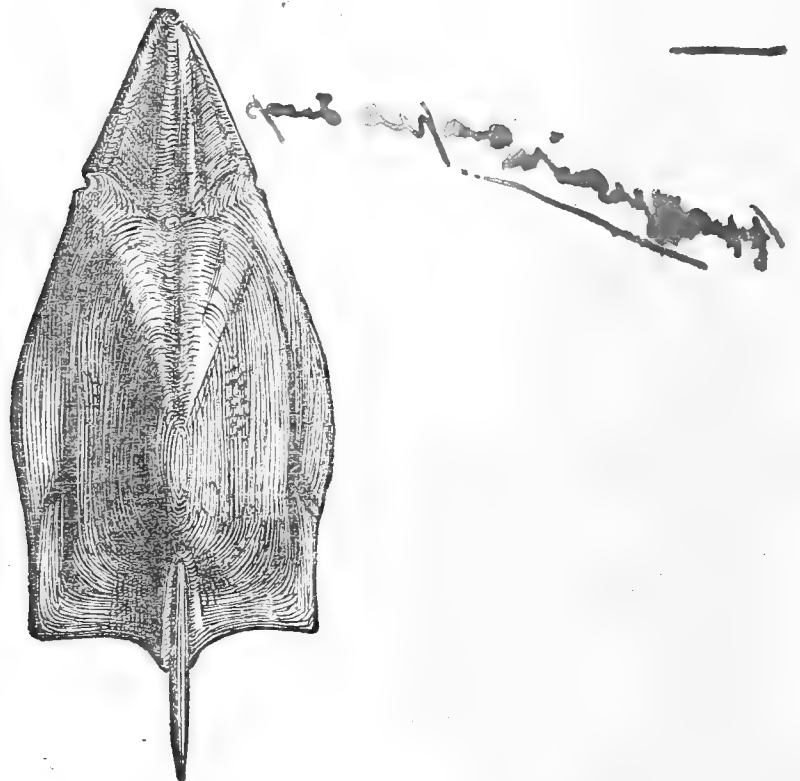
Pteraspis rostrata (Ag.).—Dorsal shield restored, after Lankester.
