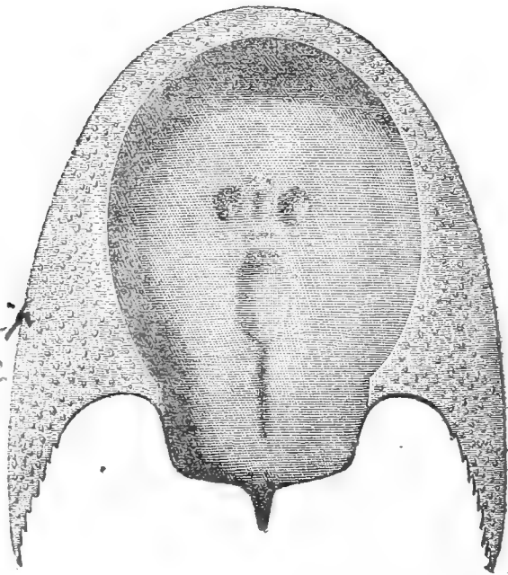
Cephalaspis .—Diagram of inferior aspect of shield, showing inferior rim; after Lankester.
