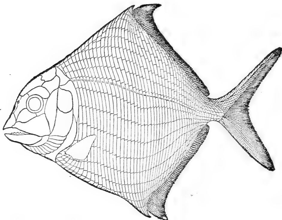
Cheirodus granulatus (Young).—Restoration by R. H. Traquair.
