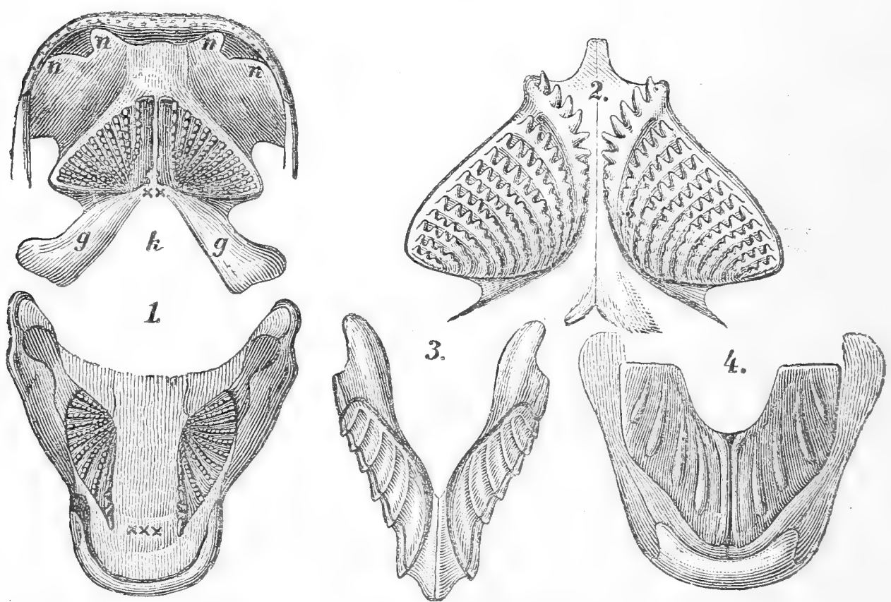
Dentition of extinct Dipnoi.—1. Dipterus valenciennesi , Sedgw. & Murch.; upper and lower jaws, nat. size. xx, upper dental plates; xxx, lower dental plates; g, upper dentigerous bones; n, narial openings. 2. Ctenodus cristatus , Ag.; upper dental plates (somewhat inaccurately drawn, the oral aspect being in reality concave), one-third nat. size. 3. Sagenodus inaequalis , Owen; lower dentition, one-half nat. size. 4. Palaeodaphus insignis , Van Ben. & De Kon.; lower dentition, one-sixth nat. size.
