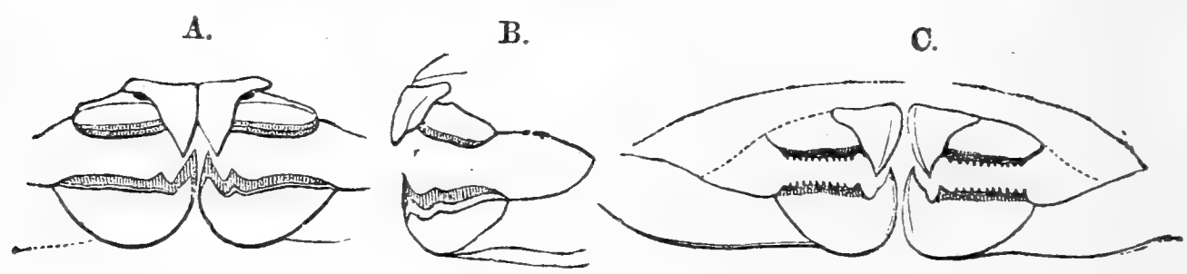
Diagrams of dentition of Dinichthys , after Newberry.—A, anterior, and B, lateral aspect of jaws of D. terrelli ; C, anterior aspect of jaws of D. hertzeri .
