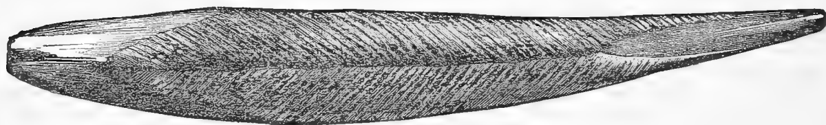
Fin-spine of Gyracanthus formosus , Ag. Coal-Measures; Dalkeith.
