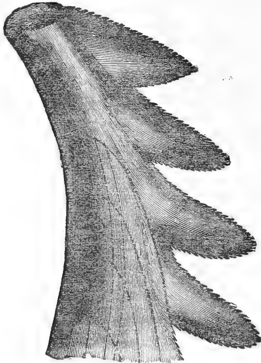
Edestus minor , Newb.—Coal-Measures, Indiana, U.S.A.
