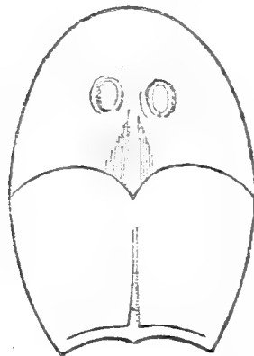
Didymaspis grindrodi , Lank.—Outline of shield, after Lankester.
