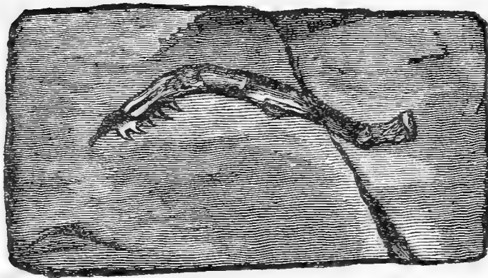
Harpacanthus fimbriatus (Stock).—M. Carb. Limest., Gilmerton. (After Traquair.)
