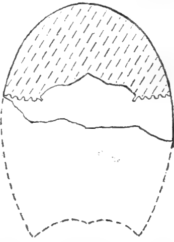
Fig. 31. Tremataspis schrenki (Pander).—Outline of shield, dorsal aspect, after F. Schmidt.
