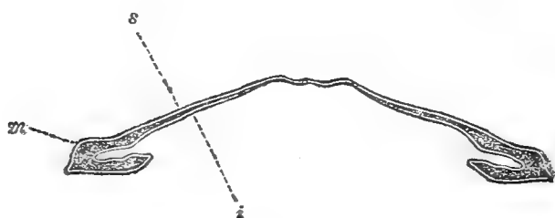
Cephalaspis . — Transverse section of shield, after Lankester. i , inferior lamina; m , margin; s , superior lamina.
