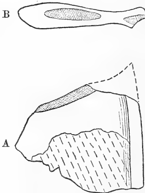
Tooth of Ptyctodus obliquus , Pander, nat. size; Devonian, Russia.—A, inner aspect, showing symphysis, the base enveloped in matrix. B, oral aspect, the tritors marked by transverse lines.
