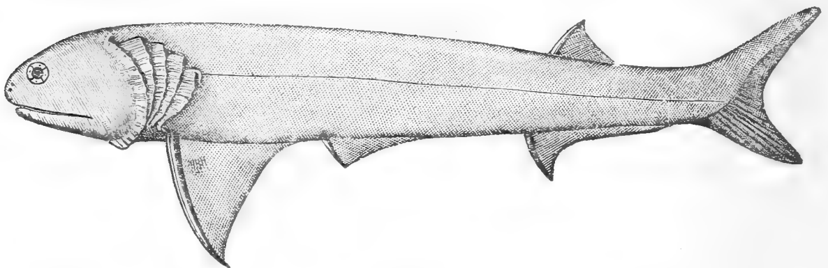
Restoration of Acanthodes wardi , Egert.—Coal-Measures, England and Scotland.
