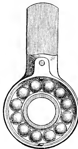
FRONT VIEW WITH CAP REMOVED.
