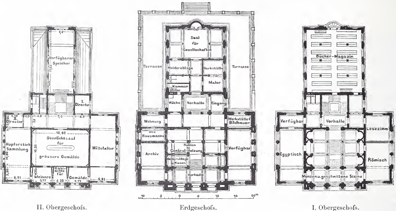
Kestner-Museum in Hannover.
