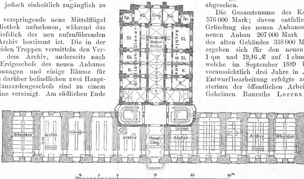
Erdgeschoss.
