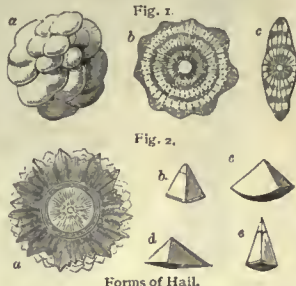
Fig. 1. a, hailstone which fell at Bonn in 1822: diameter 1 1/2 inches, weight 30 grains; b, c, sections of differently shaped hailstones which fell on the same occasion, showing the radiating nucleus and concentric layers. Fig. 2. a, section of hailstone with minute pyramids on its surface; b, c, d, e, fragments of same when burst asunder.
