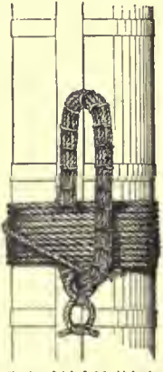
Garland (def. 8 (a)) lashed on a lower mast.
