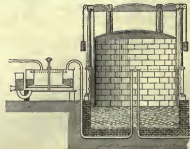
Gasometer.
