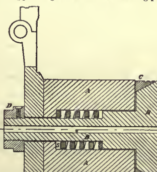
Freire Gas-check.
