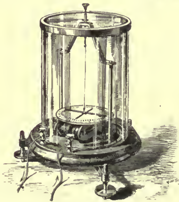
Astatic Galvanometer.
