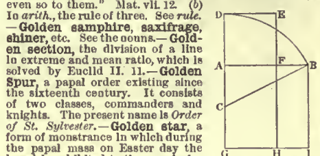
The Golden Section of Euclid II. 11. AB is the given line. The side of the square ABIG is bisected in C. CD is taken equal to BC, and the square ADEF is constructed.
