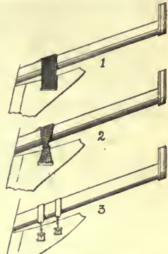
1, rope gammoning; 2, chain gammoning; 3, iron-strap gammoning.
