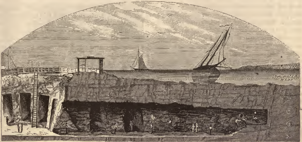
LONGITUDINAL SECTION OF GRANT HEADING.
