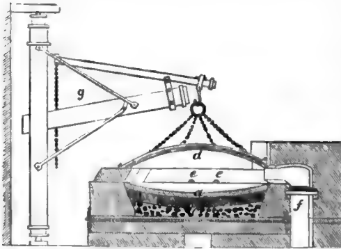
Fig. 3.—Silver Cupellation-furnace:
