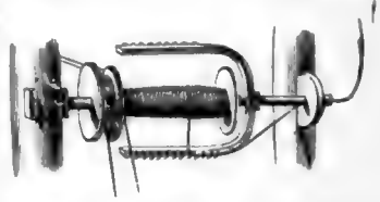
Fig. 3.—Spindle, Bobbin, and Flyer of fig. 2 on larger scale.
