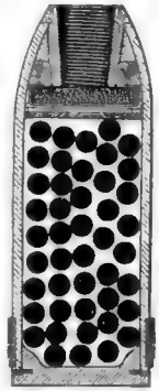
Fig. 1. Shrapnel Shell.
