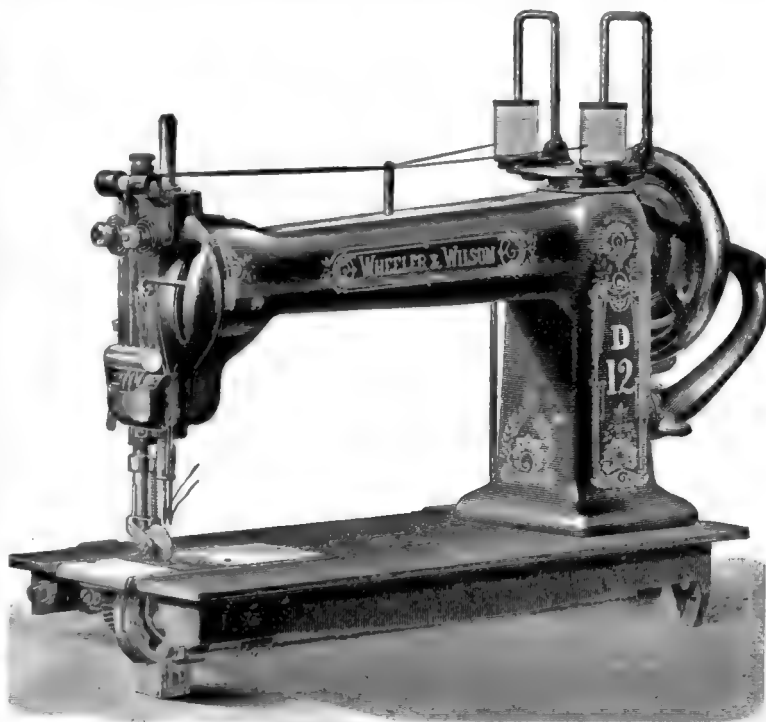
Fig. 6.—Head of Wheeler and Wilson's No. 12 fitted up with two upper threads.
