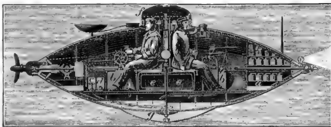
Section of the French Submarine or Surface Boat Goubet , built 1888 : a, the electric accumulators; b, tanks for compressed air; c, d, pumps; e, e, engines; f, cupola; g, the safety or emergency weight, which, in event of pumps or machines breaking down, can be detached, when the vessel at once rises to the surface. When proceeding on the surface only the cupola, f, is visible above water.
