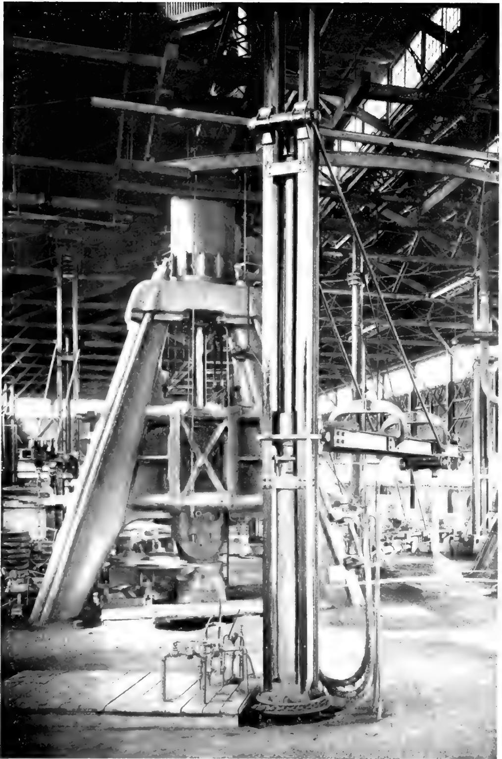
STEAM-HAMMER.
