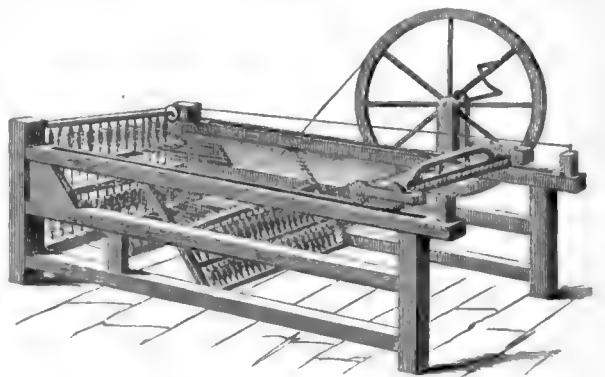
Fig. 4.—Hargreaves' Jenny.
