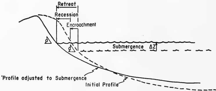
Figure 5. Terminology of retreat. \text{Retreat} = \text{encroachment} + \text{recession} \text{encroachment} = \Delta Z \cot \alpha .
