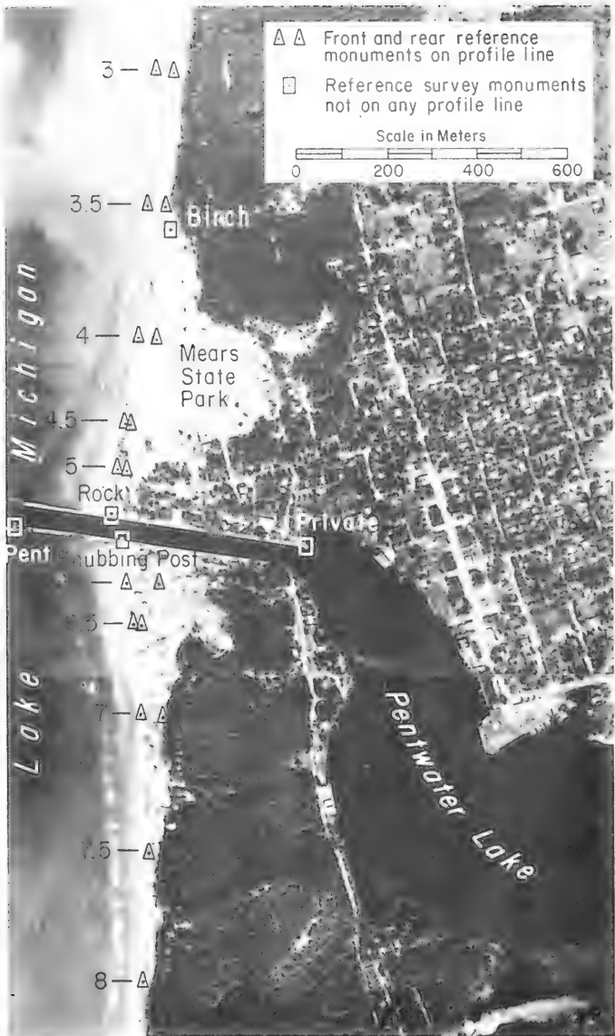
Figure 3. Profile stations in vicinity of Pentwater jetties.
