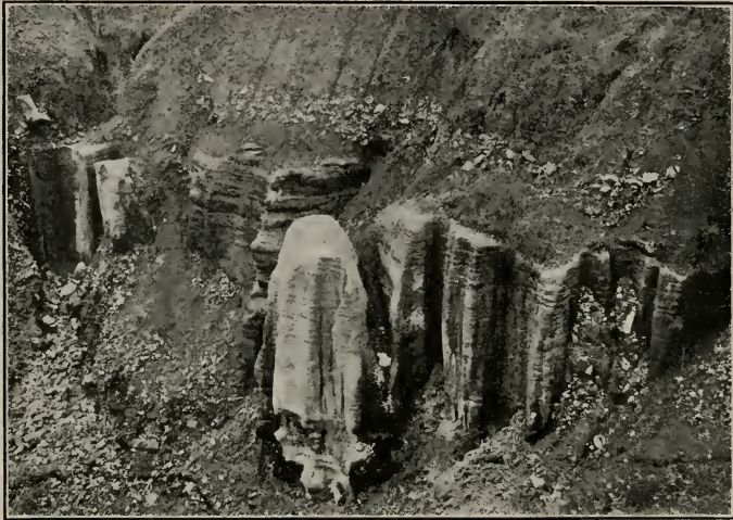
FIG. 40.—Soil-forming rock: Limestone. United States Geological Survey.
