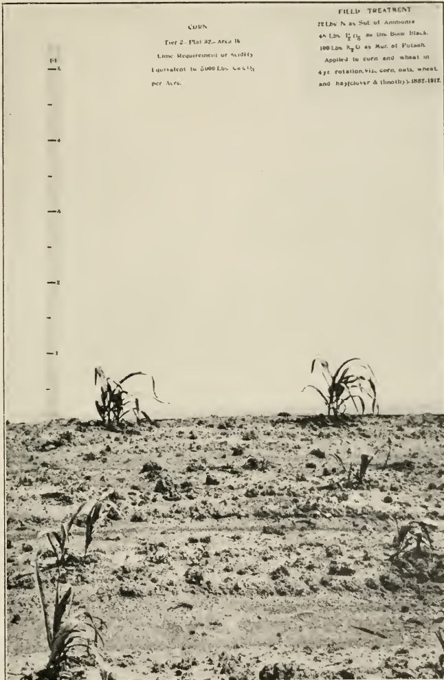
FIG. 56.—Effect of acidity resulting from use of ammonium sulphate. Corn. General fertilizer plats, Department of Agronomy, Pennsylvania Station.
