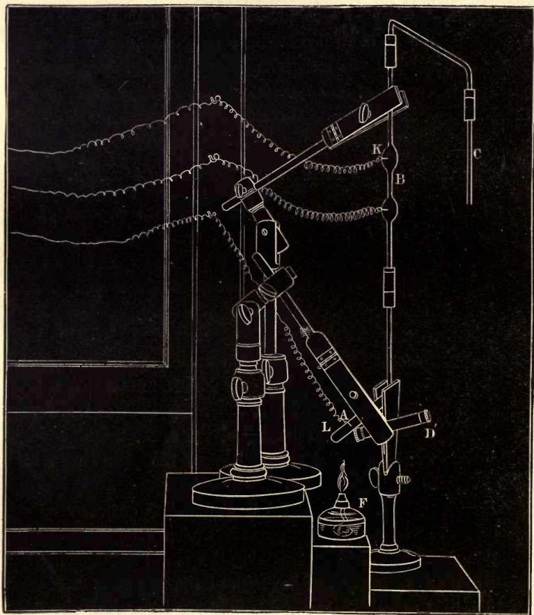
FIG. 99.—1st Form. Position of spectroscop when observing vapours close to the metal.
