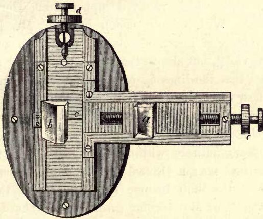
FIG. 39.— a , right-angled prism on which the image of the limb falls ; b , right-angled prism which receives light from a ; c , slit through which centre of sun is observed ; d , screw to adjust width of slit ; e , screw to adjust distance of a from b , according to the semi-diameter of solar image employed.
