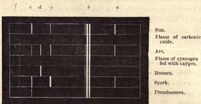
FIG. 90.—The various intensities of the lines of Magnesium as seen under different conditions
