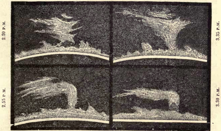
FIG. 47.—Solar prominences (Yeung), showing lateral currents.
