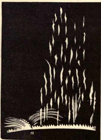
FIG. 123.—Metallic prominence, Young. Rate of ascent 400,000 miles an hour.
