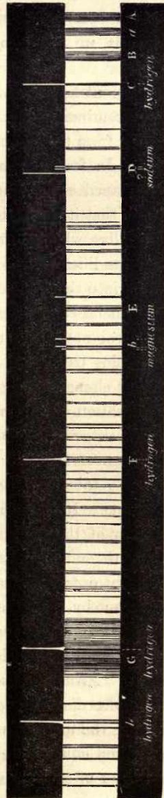
FIG. 44.—Spectrum of the sun's photosphere (below) and chromosphere (above), showing the lines ordinarily visible, and that they extend to different heights.
