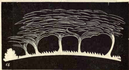
FIG. 122.—Tree-like prominences.
