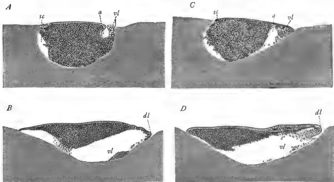
Fig. 67.—Diagrams comparing gastrulæ of Chimæra and Selachian. A and B , Earlier and later stages in gastrula of Chimæra collicii . C and D , Earlier and later gastrulæ of shark (mainly after Rückert).
