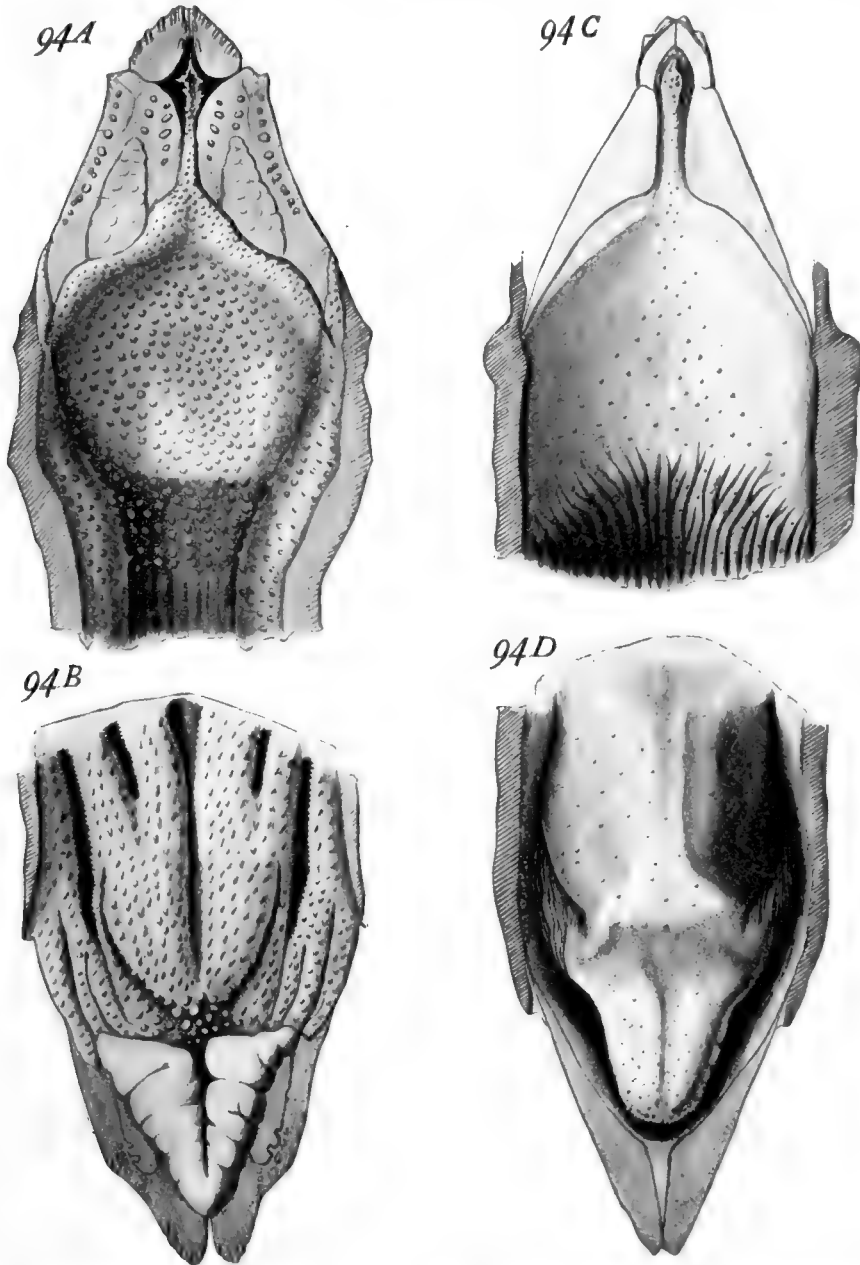
Fig. 94.—Dental plates, and roof and floor of mouth of: A, B, Harriota raleighana . C, D, Rhinochimæra pacifica .
