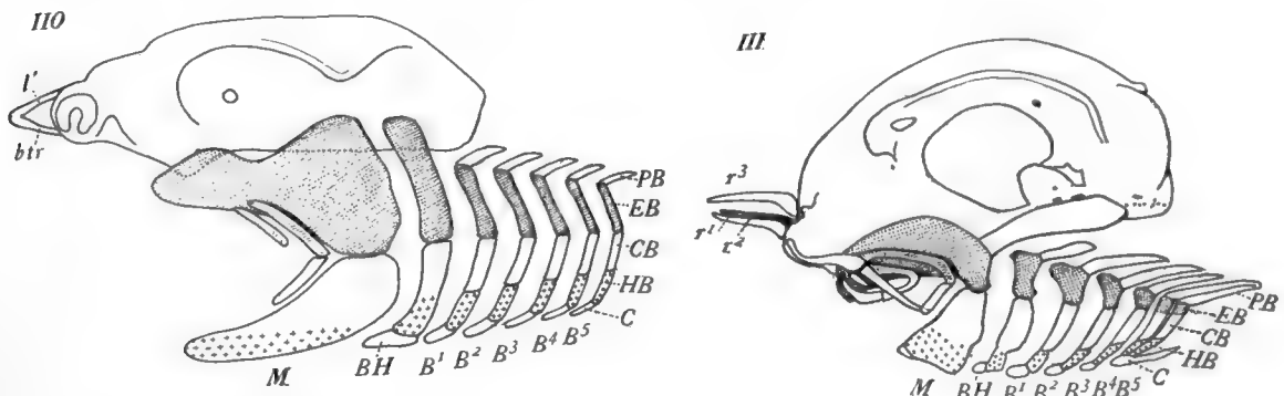
Figs. 110 and 111.—Skull and branchial arches of Shark and Chimæroid compared.
