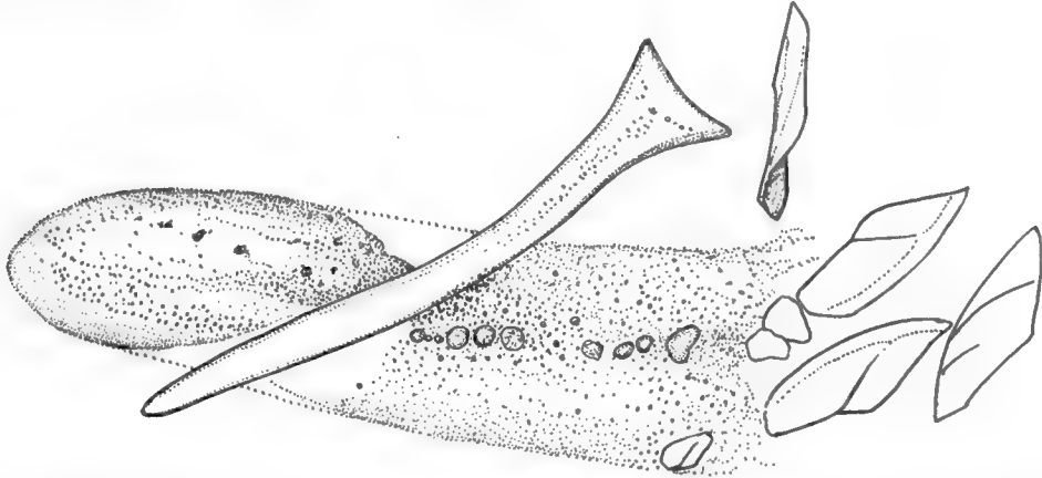
Fig. 141.— Myriacanthus granulatus . Detail of snout region.
