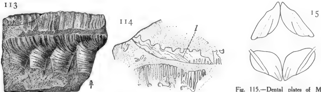
Figs. 113 and 114.—"Vertebral columns" of "Silurian Chimæroid," Dictyorhabdus priscus Walcott. The first figure after Walcott. l. , oblique laminae in the structure of the fossil, suggesting lines of growth.
