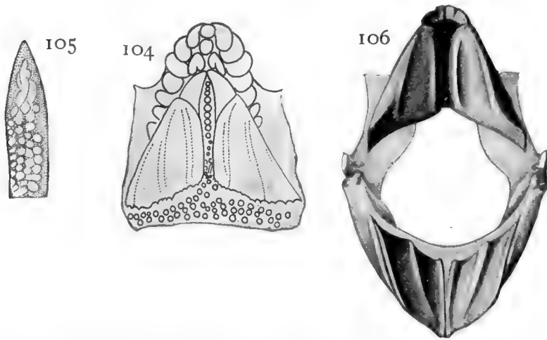
Fig. 104.— Callorhynchus callorhynchus . Dental plates and neighboring mouth parts of late embryo (about 110 mm. long). After Schauinsland.
