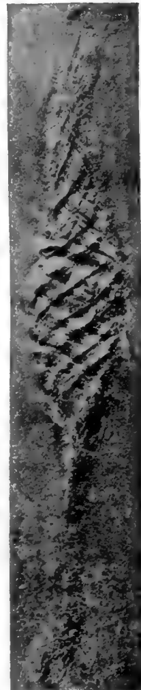
Fig. 13.—Spirangium (egg-capsule of Chimæroid?). From lithographic stone of Lerida (Spain). Jurassic. After Sauvage.
