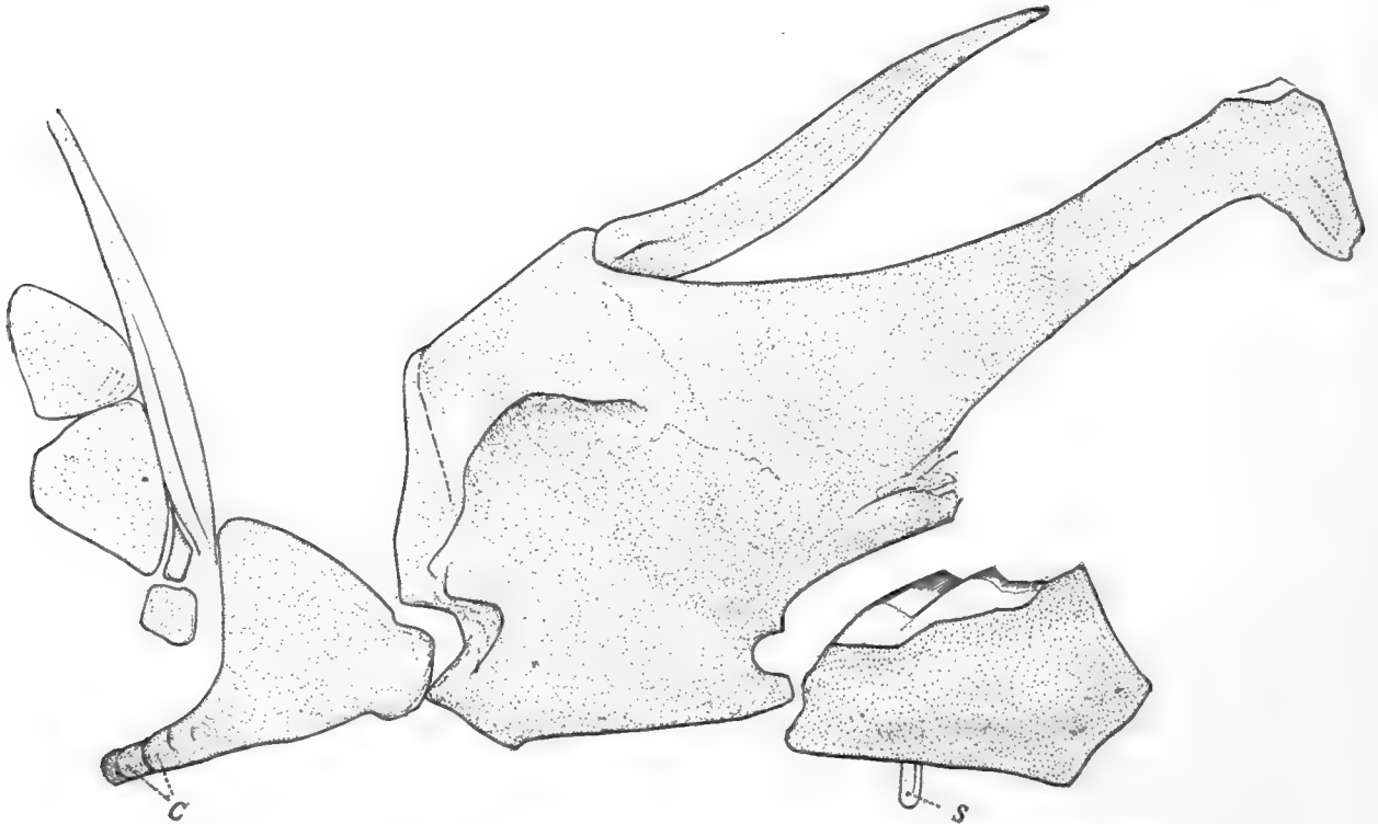
Fig. 140.—Head region of the Jurassic Chimæroid Myriacanthus. After Egerton's specimen, in British Museum. C, Centra; S, Detached ventro-median chisel-shaped "tooth."
