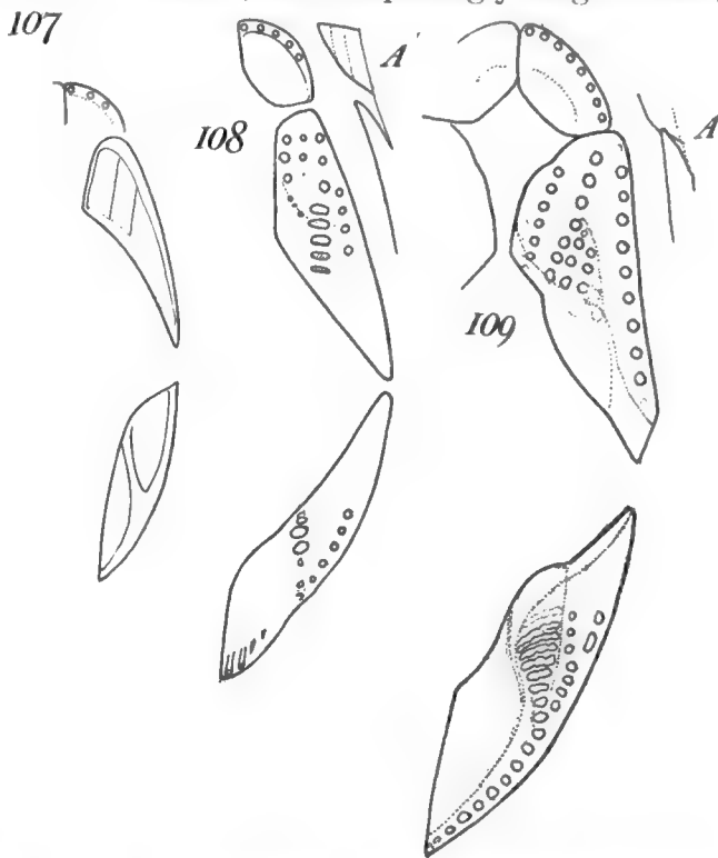
Figs. 107-109.— Harriotta raleighana . Dental plates (somewhat diagrammatic) of three individuals measuring respectively 10, 49, and 64 cm. At A the lateral aspect of the vomerine and palatine plates is given.
