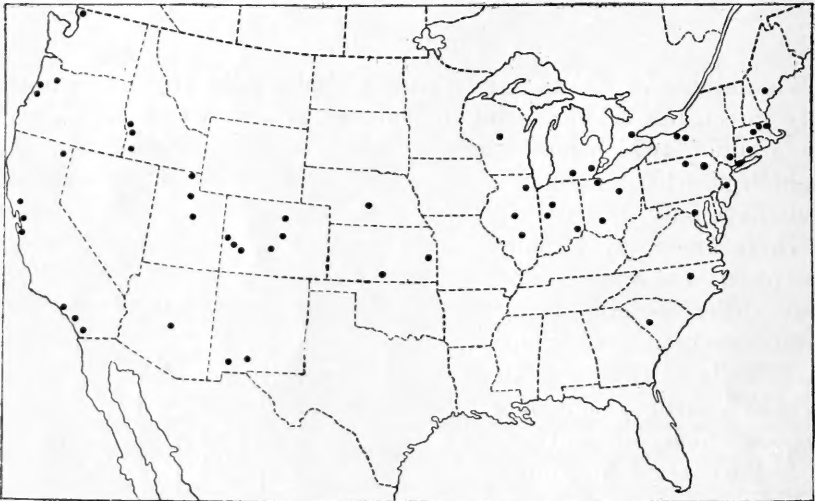
FIG. 2.—Map showing the distribution of the clover mite ( Bryobia pratensis ) in the United States in 1911. (Original.)
