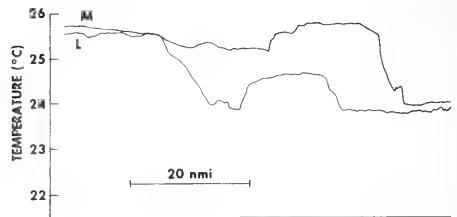
Figure 48b. Continuous sea surface analog temperature ( ^{\circ}\text{C} ) traces made across thermal discontinuities between 26 and 30 August 1979 (see figure 48). Values to the left in traces I, J, and K give temperatures in cool, upwelled water of coastal origin. Values to the left in traces L and M give temperatures in the interior of the Socotra Eddy
