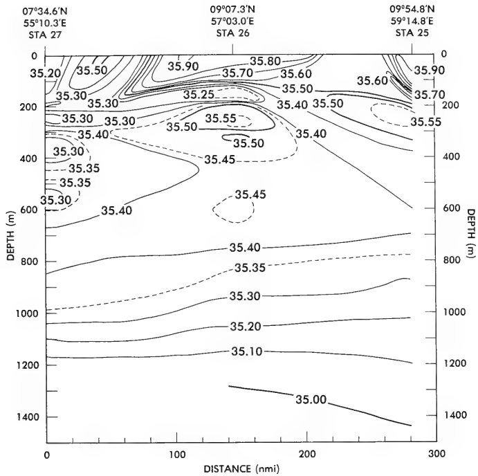
Figure 47. Salinities ( ^{\circ}/_{\text{00}} ) along Section 9, USNS WILKES, 31 August - 2 September 1979
