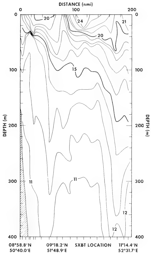
Figure 10. XBT Temperature ( ^{\circ}\text{C} ) Section 5, 26 - 27 August 1979 (see figure 5)
