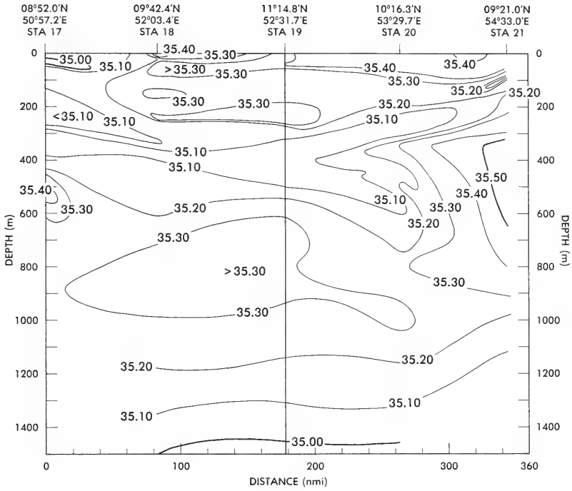
Figure 43. Salinities ( ^{\circ}/_{\infty} ) along Section 5 and 6. Section 5 is left of solid line at Station 19. USNS WILKES, 26 - 28 August 1979
