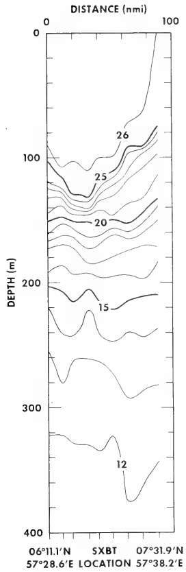
Figure 8. XBT Temperature ( ^{\circ} C) Section 3, 22 - 23 August 1979 (see figure 5)
